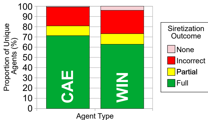
Figure 10. Distribution of the four possible outcomes of the siretization process for the annotated SIRETs (the exact values are shown in Table 31).
