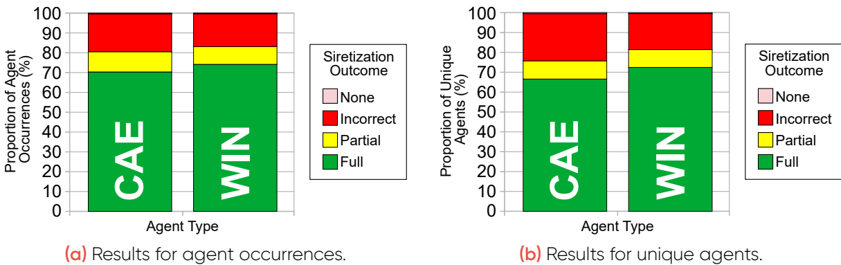
Figure 9. Distribution of the four possible outcomes of the sirezitization process for the predefined SIRETs.
