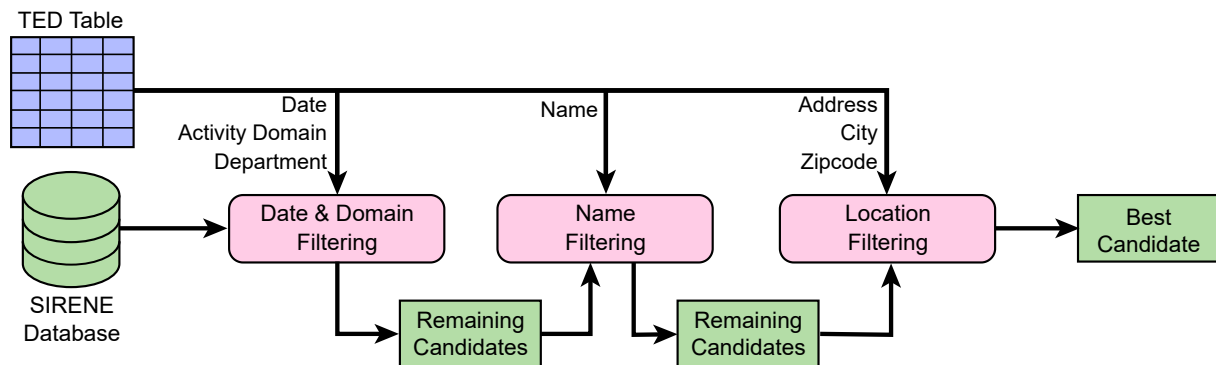
Figure 8. Successive filtering phases of the siretization process. The square boxes represent data, and the round ones processing steps.
