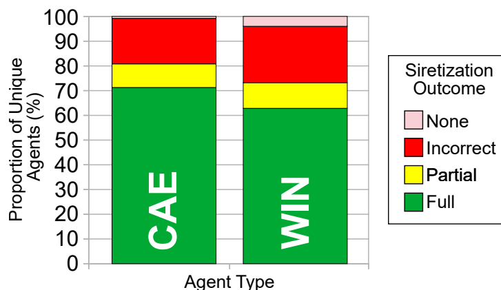
Figure 10. Distribution of the four possible outcomes of the sirezitization process for the annotated SIRETs (the exact values are shown in Table 31).
