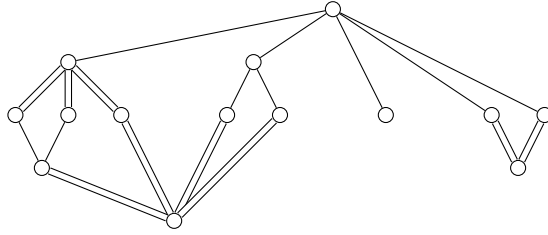
FIGURE 4.3. Example of an element of \mathcal{C} of size 14.
