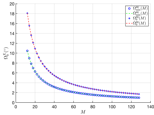
Fig. 6 \Omega_{\min/0}^{80}(M) and \tilde{\Omega}_{\min/0}^{80}(M) for M \in [12, 128]
