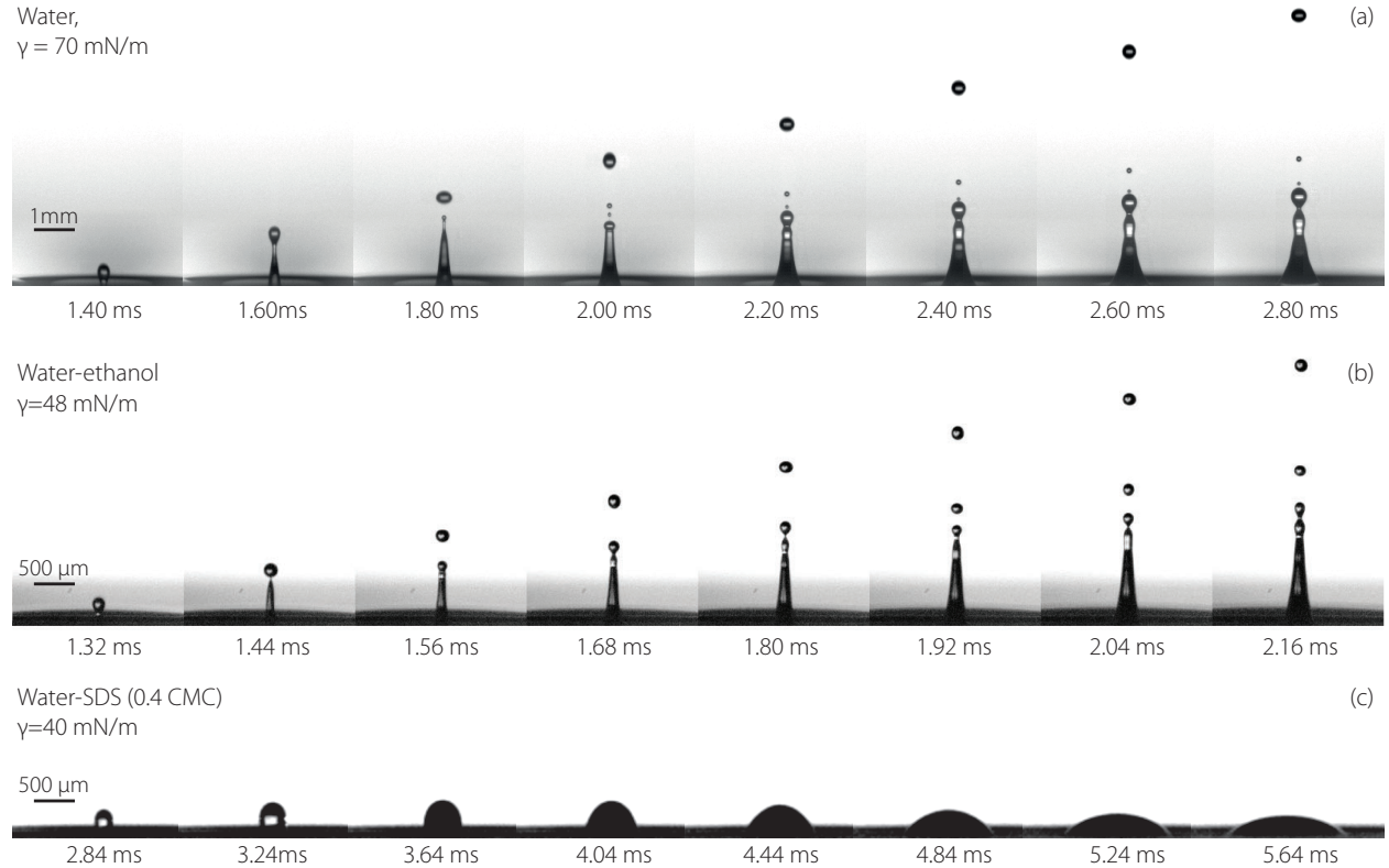
FIG. 1. Sequences of bursting bubbles (bubbles start to burst at 0 ms) with comparable radius in three different liquids : (a) water, \gamma = 70 \text{ mN}\cdot\text{m}^{-1} , R = 830 \mu\text{m} ; (b) water-ethanol solution with respectively 89.5% and 10.5% of total weight, \gamma = 48 \text{ mN}\cdot\text{m}^{-1} , R = 830 \mu\text{m} ; (c) water-SDS solution with 3.4 mM of SDS, \gamma = 40 \text{ mN}\cdot\text{m}^{-1} , R = 840 \mu\text{m} . The surfactants have a strong influence on the jet dynamics, independently of their influence on the surface tension. The time and space scales of the sequences (a) and (b) have been chosen in order to show the similarity between the two dynamics.
