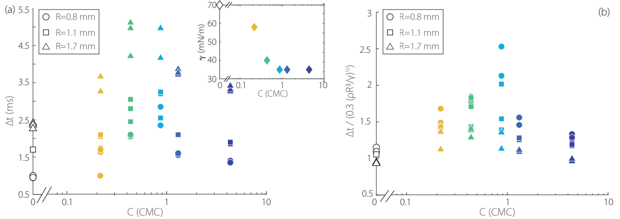
FIG. 2. (a) Bubble collapsing time \Delta t for three different bubble radii R = 0.8 \pm 0.1 \text{ mm} (circle), 1.1 \pm 0.1 \text{ mm} (square) and 1.7 \pm 0.1 \text{ mm} (triangle), as a function of the surfactant concentration, adimensionalized using the critical micelle concentration (CMC). The CMC is taken equal to 8 mM [33]. Inset: for each solution the surface tension is measured using the pendant drop technique and reported as a function of the surfactant concentration. (b) Collapsing time, \Delta t , normalized by the capillaro-inertial time scale, \sqrt{\rho R^3 / \gamma} , as a function of the dimensionless surfactant concentration, for three different bubble radii R = 0.8 \pm 0.1 , 1.1 \pm 0.1 and 1.7 \pm 0.1 \text{ mm} . The 0.3 prefactor is added in the normalization of \Delta t in order to have the dimensionless collapsing time equal to one. The color of the markers is associated to the surfactant concentration in the liquid.
