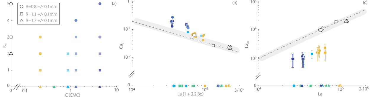
FIG. 3. (a) Number of ejected drops as a function of the SDS concentration. The opacity of the symbols has been decreased so that the superposition of symbols appears darker and every data point can be seen. (b) Capillary number of the first ejected drop as a function of La(1+2.2Bo) . The dashed line represents the relation : Ca_{d1} = 19(1 + 2.2Bo)^{-3/4}La^{-3/4}(500^{-1/2} - La^{-1/2})^{-3/4} used in [22] (Eq. 5) and in [46] (Eq. 6) and based on the scaling law proposed by Gañán-Calvo (2017) [12]. (c) Laplace number of the first ejected drop as function of the Laplace number of initial bubble. The dashed line represents the scaling proposed by Gañán-Calvo (2017) [12] : La_{d1} = 0.6[\sqrt{La}(\sqrt{La/500} - 1)]^{5/4} and already used in [22] (Eq. 7). In all graphs color codes for the SDS concentration and symbol codes for the bubble size. The thickness of the grey zone simply reproduces the dispersion of the experimental and numerical values appearing in the corresponding figures of Berny et al. [22].
