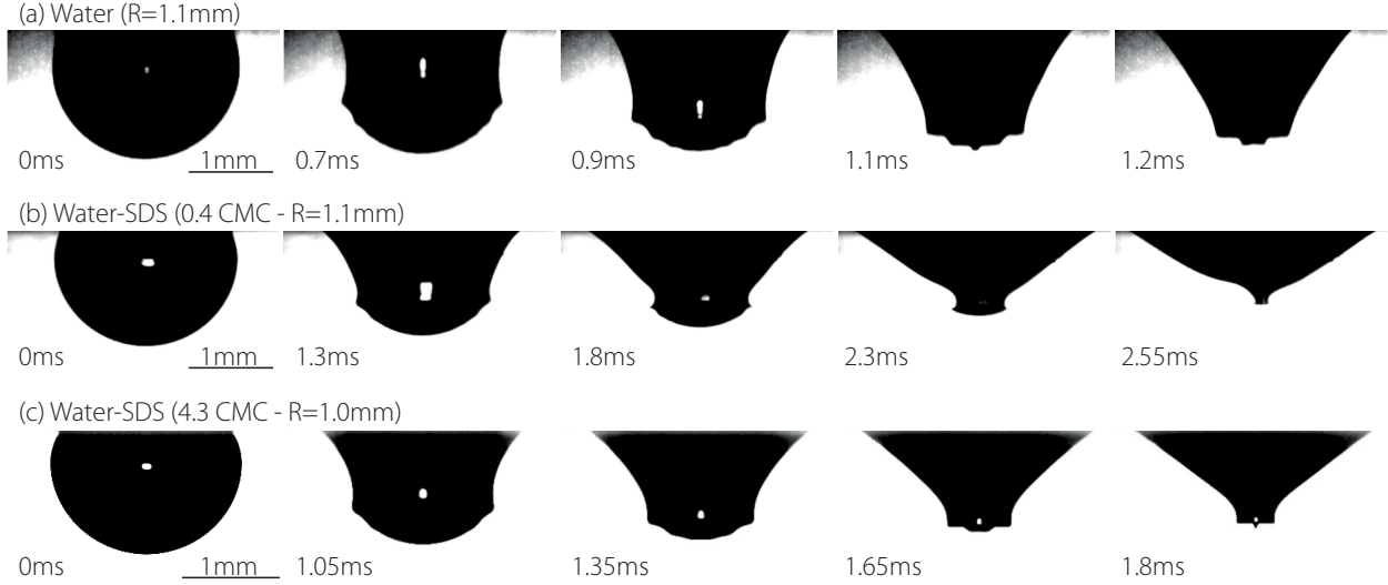
FIG. 4. Sequences showing the collapse of the submerged cavity for bubbles with almost the same radius in three different liquids: (a) water, \gamma = 70 \text{ mN}\cdot\text{m}^{-1} , R = 1.1 \text{ mm} , (b) water-SDS solution at 0.4 CMC, R = 1.1 \text{ mm} , (c) water-SDS solution at 4.3 CMC, R = 1.0 \text{ mm} . The time scale of the three sequences has been chosen in order to compare the whole dynamics of the collapsing cavity, from cap film rupture up to cavity reversal.
