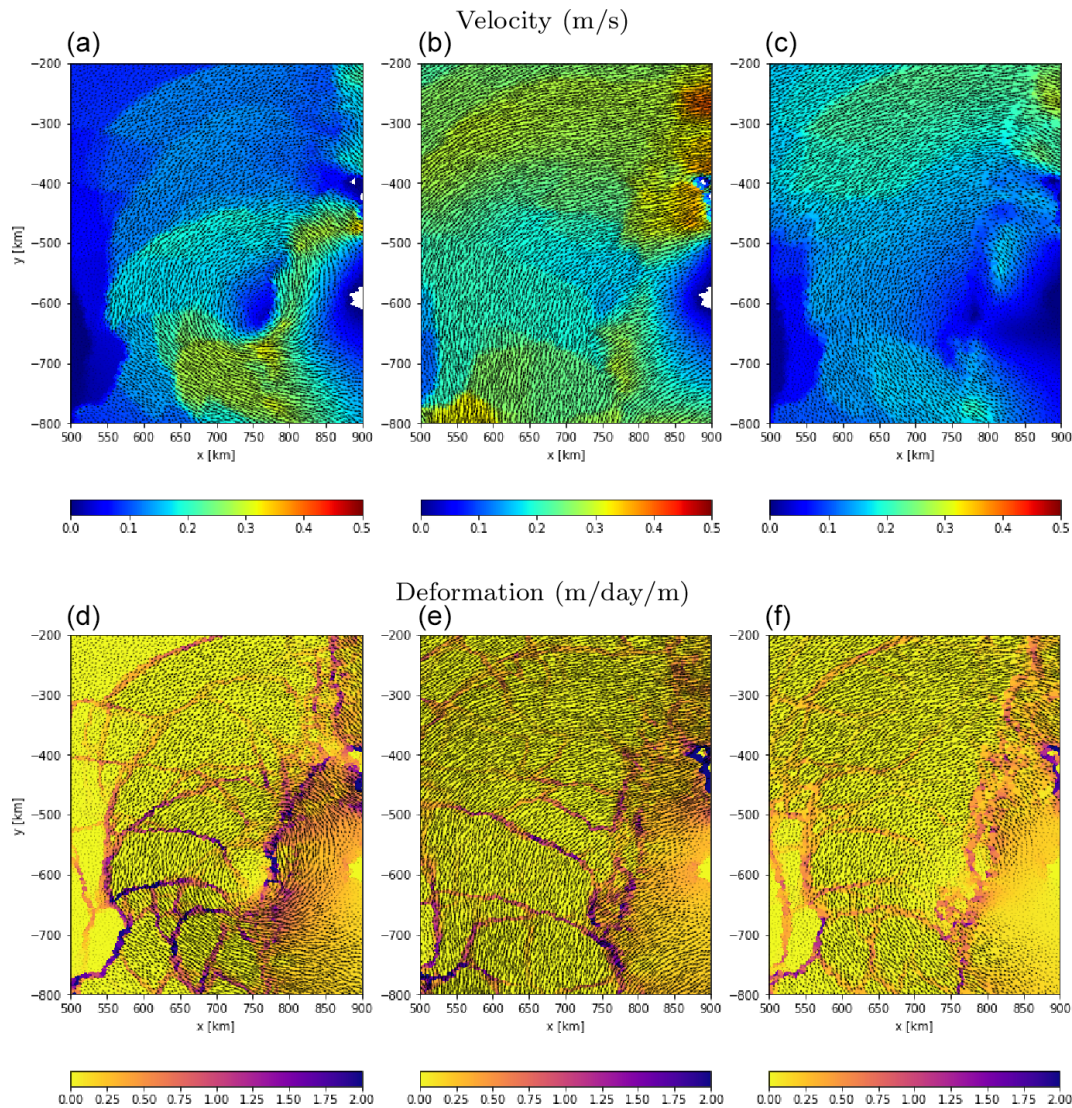
Figure 7. Instantaneous sea-ice velocities at two epochs separated by a day (a, b) and daily integrated velocities (c) as estimated from the neXtSIM sea-ice model. At the bottom is the associated deformation.
