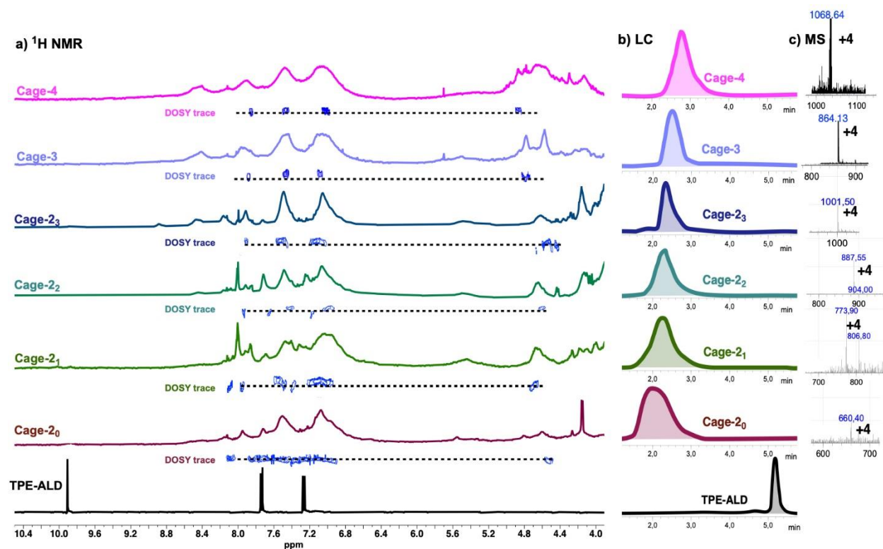
Figure 1. Formation of molecular cages by hierarchical covalent self-assembly. (a) ^1\text{H} NMR (600 MHz, \text{DMSO-}d_6 ) of reactions mixtures with, below, the extracted DOSY NMR spectrum; (b) HPLC chromatograms; (c) extracted mass spectra.
