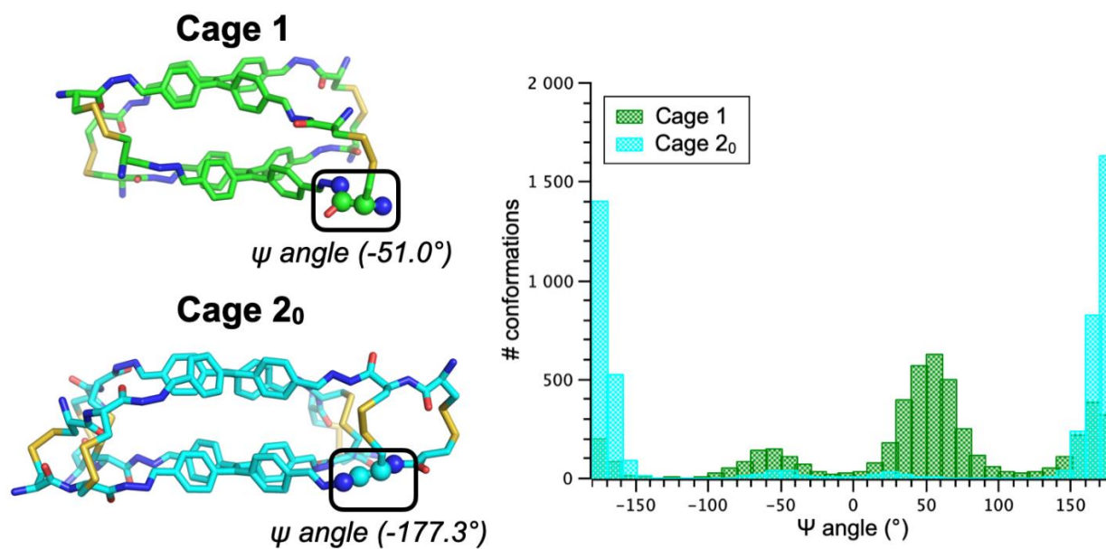
Figure 4. Side view of the final MD snapshots of Cage 1 and Cage 2 0 . Hydrogen atoms were omitted for clarity. The atoms represented in spheres are related to a specific \Psi dihedral angle, for which the distributions issued from the MD simulations are shown on the right. Cage 2 0 has more extended arms with the planarization of \Psi dihedral angle compared to Cage 1 .
