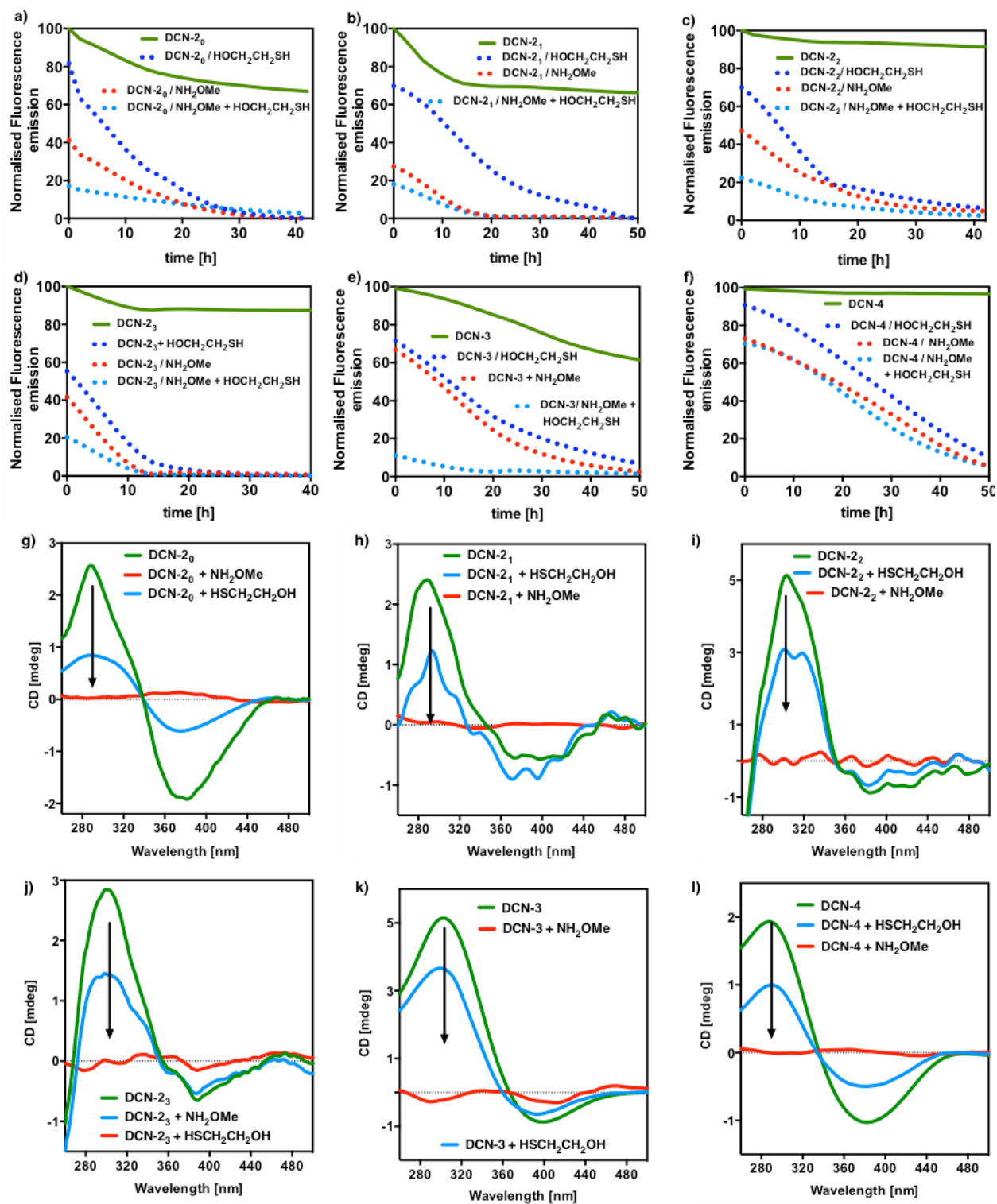
Figure 7. Chemically-controlled degradation of DCNs, made from different cysteine-rich C-hydrazide peptides, monitored by fluorescence (a-f) and circular dichroism (g-l) spectroscopies upon addition of methoxyamine (20 equiv.) and/or \beta -mercaptoethanol (100 equiv.) in 94/6
