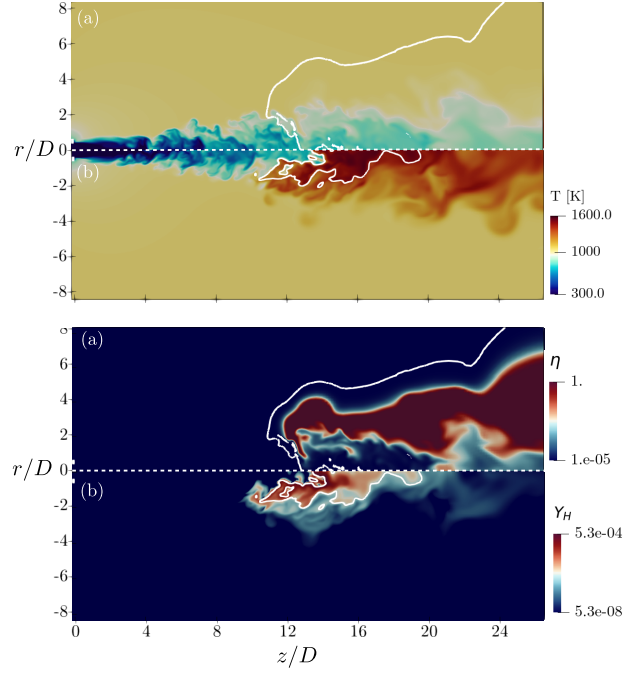
Figure 11: Two dimensional cross-section of instantaneous flow field. Temperature and \eta are presented with (a) compared with the reactive test case (b). Auto-ignition condition ( \eta = Y_{\text{H}_2}^0/10000 ) is presented with white line contours for non reactive and Y_{\text{OH}} = 600 PPM as taken from Cabra et al. [10].
