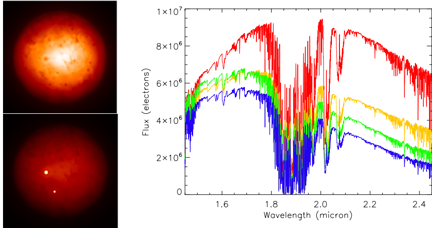
Figure 5: Simulated images of Io, observed with HARMONI at 4\times 4 mas scale, without deconvolution. The bottom image shows two volcanic hot spots that dominate the near-IR emission, while the top image is in a quiescent state. Simulated spectra of four hot-spots at different temperatures ranging from 600 K to 1200 K are also shown.
