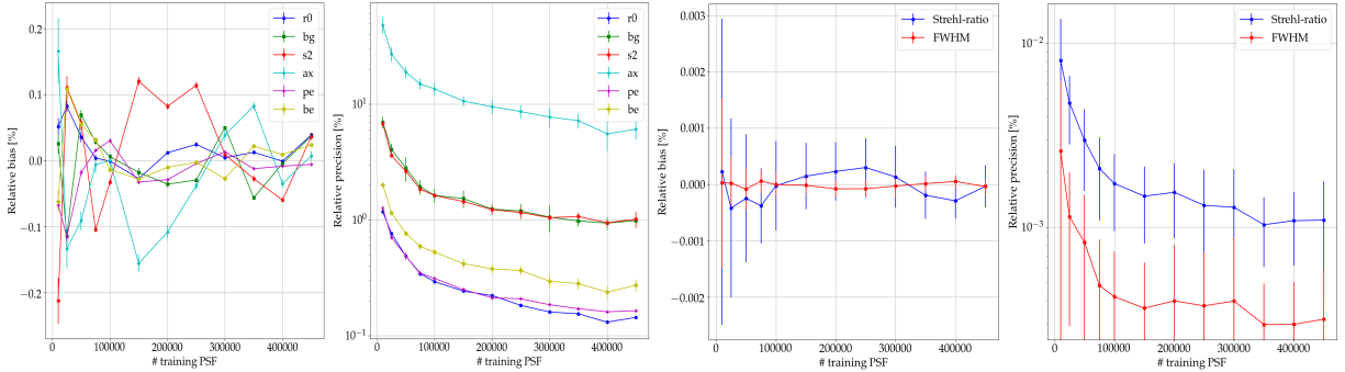
Figure 3. Left : Bias and StD for the 6 parameter estimates; Right : PSF-based metrics (Strehl ratio and FWHM). In both cases, the results are given as a function of the number of PSFs used during the training step.
