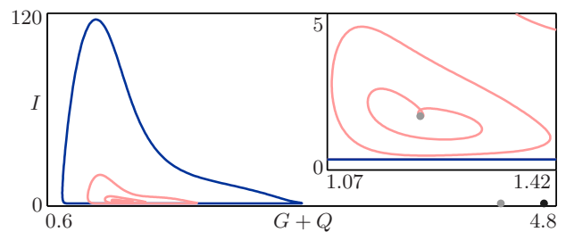
FIG. 3. Phase portrait of (1) in the (G + Q, I) -plane, for A = 2.7 , R_{sp} = 0 and n_G = 0 . Dots are equilibria and closed curves are periodic orbits. Stable and unstable periodic orbits are represented in blue (dark grey) and pink (light grey), respectively; stable and unstable equilibria are represented in black and grey, respectively.
