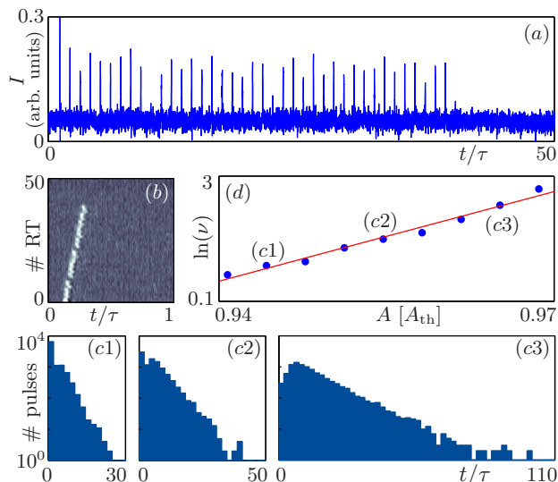
FIG. 2. Experimental measurements: (a) Typical pulse train, with finite duration. (b) Pseudo-space mapping of the time trace (see text). (c) Log-scale histograms of the number of pulses in 20,000 recorded trains, for pump currents of 94.4%, 95.4% and 96.5% of the laser threshold A_{\text{th}} . (d) Logarithm of the corresponding decay rate \nu (scaled to the feedback delay \tau ) versus scaled pump A .
