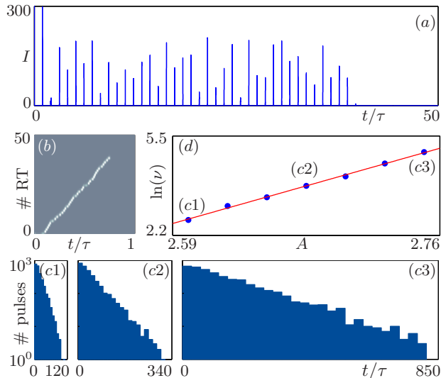
FIG. 4. Simulation of system (1) with noise: (a) typical time trace for A = 2.7 , n_G = 0.025 , \kappa = 0.04 and \tau = 1000 and (b) its representation in the pseudo-space map. (c) Log-scale histograms of the number of pulses in 5000 simulated trains, for three values of A . (d) Logarithm of \nu versus A .
