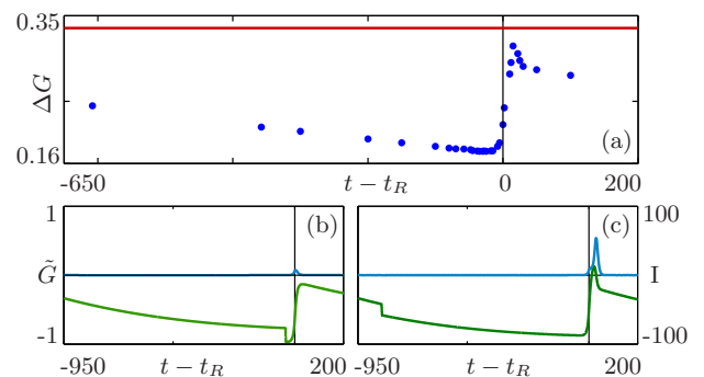
FIG. 5. Evaluation of noise bias: (a) Minimal gain perturbations \Delta G_{off} (blue dots) and \Delta G_{on} (red line) required to terminate a pulse train and trigger a first pulse, respectively, versus t - t_R , with t_R the reinjection time of the previous pulse. (b)–(c) Net gain \tilde{G} (green lower line) and intensity I (blue upper line) versus t - t_R , for a perturbation \Delta G = -0.2 at t - t_R = -35 and at t - t_R = -850 , respectively.
