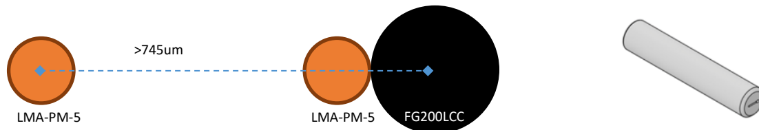
Figure 4-3: (Left) Fibre bundle output geometry showing the MM fibre (black) and SM fibre (orange). (Right) custom ferrule by Northern Light Optical.
