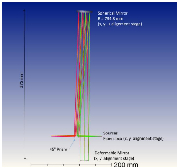
Figure 3-1: AOCU optical design (left) and image quality over a field of view of 1 mm 2 .
