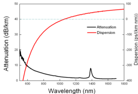
Figure 4-2: Attenuation of LMA-5 as a function of wavelength
