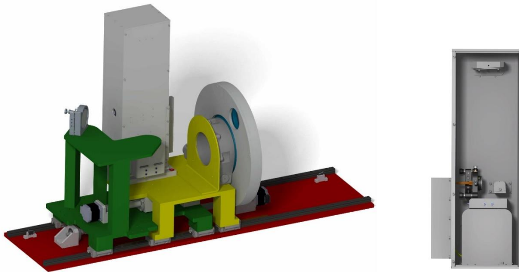
Figure 2-4: Illustration of the AOCU in its context (left), and the AOCU box showing the optical bench.
