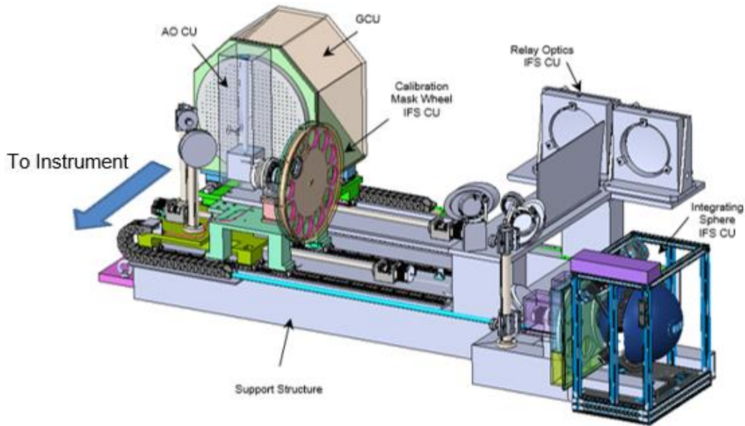
Figure 2-2: CM main structure and components, showing the location of the AO Calibration Unit in transparency.
