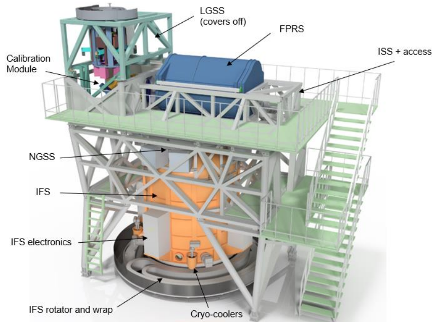
Figure 2-1: Rendering of HARMONI structure highlighting some key elements and modules. The Calibration Module can be deployed into the instrument focal plane to inject calibration light into the rest of the system.
