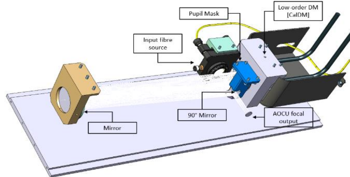
Figure 2-3: AOCU design with main elements highlighted.
