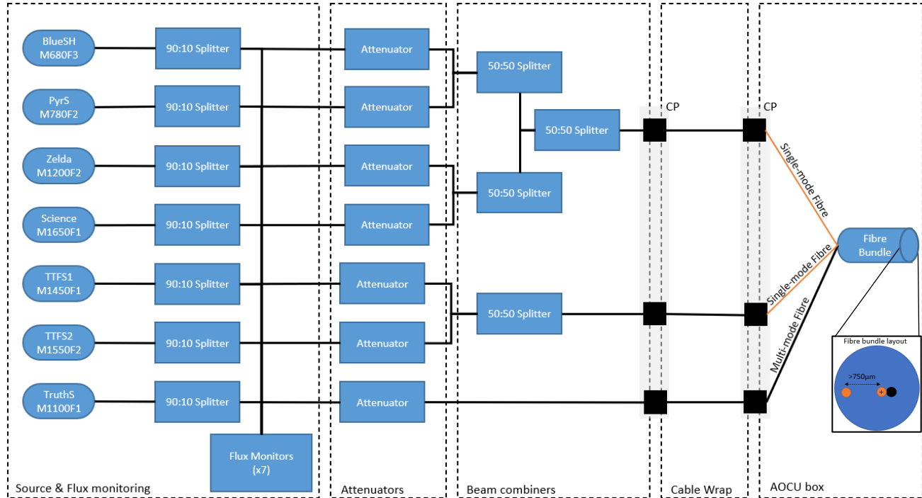
Figure 4-1: General overview of the illumination system architecture. (CP: Connector Panel).
