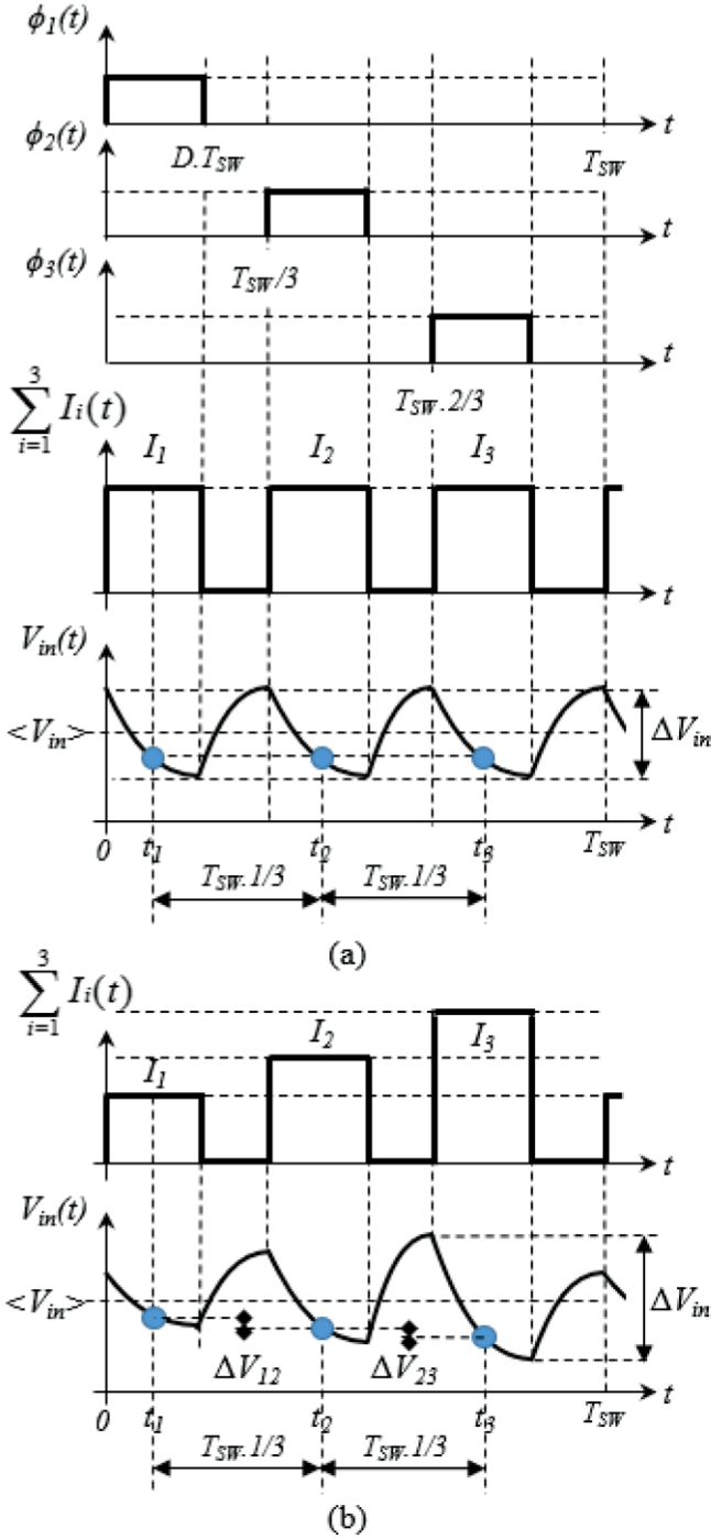
Fig. 2: a) Balanced b) Unbalanced leg currents principle of the distributed balancing consists of ensuring that each LC takes N samples from the signal V_{in} as follows:
