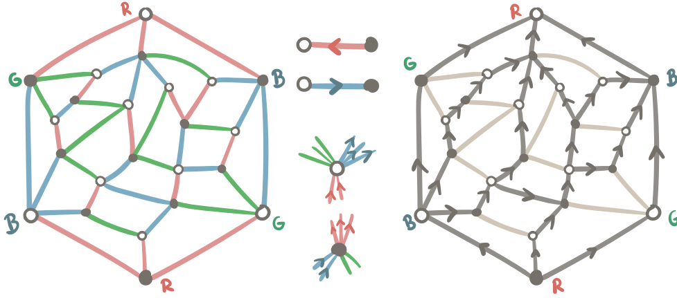
Figure 6: On the left a Schnyder labeling (with non-isolated outer G vertices), and on the right the corresponding S -transverse plane bipolar orientation.
