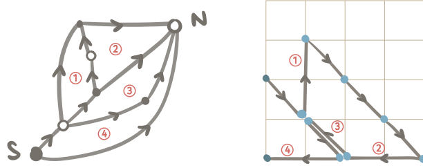
Figure 7: A bipartite plane bipolar orientation, and the corresponding even tandem walk through the KMSW bijection.
