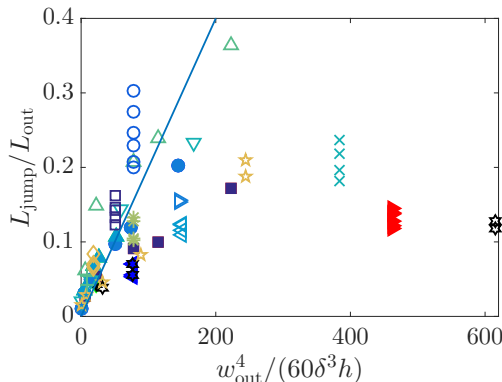
FIGURE 11. Plot of the ratio L_{\text{jump}}/L_{\text{out}} as a function of w_{\text{out}}^4/(60\delta^3h) ; see captions of figures 9 and 10 for the meaning of the various symbols. The straight line is the linear law of slope 2 \times 10^{-3} .
