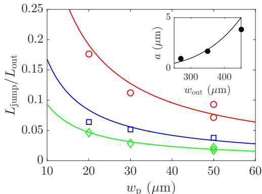
FIGURE 12. Plot of the ratio L_{\text{jump}}/L_{\text{out}} as a function of the constriction width w_p for three different channel widths: w_{\text{out}} = 270 ( \diamond ), 350 ( \square ) and 450 \mu\text{m} ( \circ ), with h = 67 \mu\text{m} , H = 95 \mu\text{m} and L_{\text{out}} = 11 or 22 mm. The straight lines correspond to the best inverse fits: L_{\text{jump}}/L_{\text{out}} = a/w_p , with a a fit parameter. Inset: plot of a as a function of w_{\text{out}} . The curve is the best fit by the formula a = cw_{\text{out}}^4 , with c = 1.2 \times 10^{-10} \mu\text{m}^{-3} as best fitting parameter.
