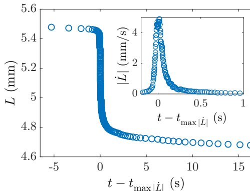
FIGURE 14. Plot of the water length L as a function of time t - t_{\max|\dot{L}|} in a channel of geometrical parameters L_{\text{out}} = 5.5 mm, L_p = 1 mm, w_{\text{out}} = 390 \mu\text{m} , w_p = 30 \mu\text{m} , h = 65 \mu\text{m} and H = 95 \mu\text{m} . Inset: plot of the corresponding meniscus velocity |\dot{L}| as a function of time in the fastest phase. The time t_{\max|\dot{L}|} is the instant where the velocity reaches its maximal value.
