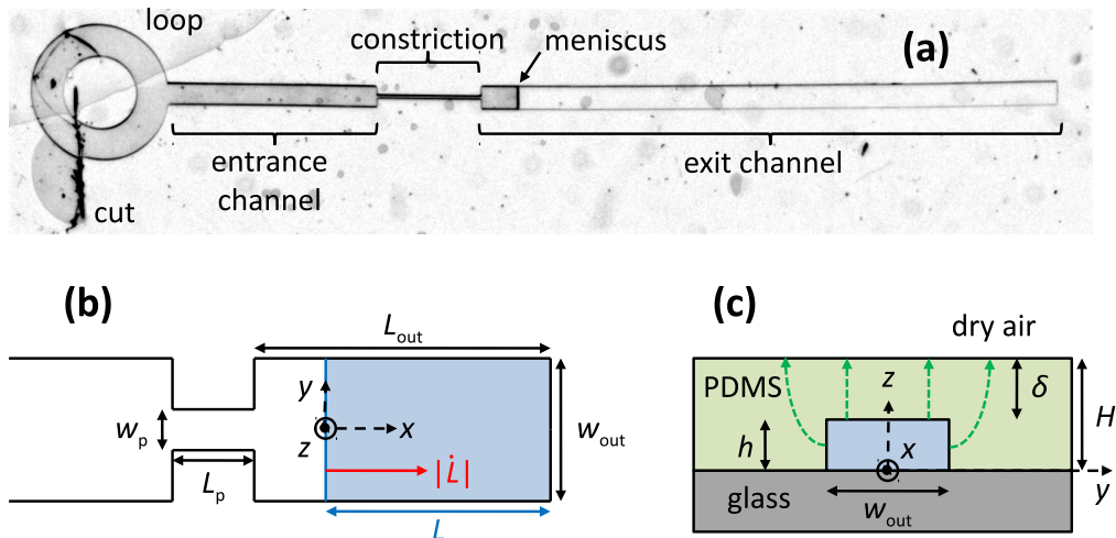
FIGURE 1. (a) Snapshot of the channel, with its different elements. Sketch of the channel (not to scale): (b) top view (excluding the loop), (c) side view across the channel. The top view shows the constriction of length L_p and width w_p inside the channel of width w_{out} . The exit channel, i.e. the channel portion after the constriction, has a length L_{out} . A meniscus, depicted as a blue line across the channel, separates the water-filled part of the channel (right of the meniscus, blue shade in panel b) of length L from the air-filled part (left of the meniscus). The velocity of the meniscus |\dot{L}| is indicated with a red arrow in panel (b); the meniscus motion is due to the loss of water induced by a pervaporation flux across PDMS, sketched by the green dotted arrows in panel (c).
