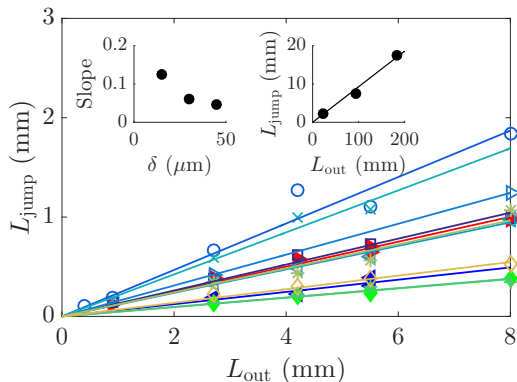
FIGURE 9. Plot of the jump length L_{\text{jump}} as a function of the length of the exit channel L_{\text{out}} . Filled symbols are for fixed values of both the exit channel width w_{\text{out}} = 300 \mu\text{m} and channel height h = 65 \mu\text{m} , and for three values of the upper wall thickness: \delta = 15 \mu\text{m} ( \blacktriangleright ), 30 \mu\text{m} ( \blacktriangleleft ) and 45 \mu\text{m} ( \blacklozenge ). Other symbols are for fixed channel width w_{\text{out}} = 300 \mu\text{m} , and for couples of values of (h, \delta) equal (in \mu\text{m} ) to: 53, 37 ( \square ); 44, 34 ( \circ ); 53, 26 ( \triangleright ); 65, 34 ( \triangleleft ); 44, 20 ( \times ); 100, 54 ( + ); 53, 323 ( * ); 53, 52 ( \diamond ). Straight lines are the best linear fits of the each series of data. The left inset shows the best fitting slope as a function of \delta for fixed values of both the exit channel width w_{\text{out}} = 300 \mu\text{m} and channel height h = 65 \mu\text{m} . The right inset is a plot of the jump length L_{\text{jump}} as a function of the length of the exit channel L_{\text{out}} in long channels of width w_{\text{out}} = 350 \mu\text{m} , for h = 67 \mu\text{m} and H = 111 \mu\text{m} .
