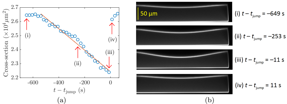
FIGURE 4. (a) Plot of the cross-section of the channel S as a function of time in a channel of geometrical parameters L_{\text{out}} = 5.5 mm, L_p = 1 mm, w_{\text{out}} = 390 \mu\text{m} , w_p = 30 \mu\text{m} , h = 65 \mu\text{m} and H = 95 \mu\text{m} . The time here is defined with respect to the instant of the jump t_{\text{jump}} , assumed to be half way between the times of the two images immediately before and after the jump. The straight line is a linear fit over the time interval where the cross-section decreases. Arrows with labels refer to the photographs taken with the confocal microscope displayed in panel (b). The boundary of the channel cross-section appears in light shade; notice that a tiny part of the cross-section is cut at the left of the photographs, owing to limitations of the horizontal field of view of the confocal microscope.
