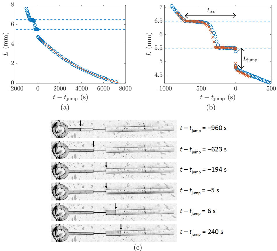
FIGURE 2. (a) Plot of the water length L as a function of time t - t_{\text{jump}} in a channel of geometrical parameters L_{\text{out}} = 5.5 mm, L_p = 1 mm, w_{\text{out}} = 390 \mu\text{m} , w_p = 30 \mu\text{m} , h = 65 \mu\text{m} and H = 95 \mu\text{m} , for a relative humidity \text{RH} = 0.25 . The time t_{\text{jump}} is the instant where the meniscus abruptly jumps inside the exit channel. The curve is a fit after the jump by the truncated exponential law (3.1), with \tau = 5.65 \times 10^3 s and L_g = 1.71 mm as fitting parameters. (b) Zoom in the constriction of the experiment presented in panel (a) ( \circ ), and of a second realisation of the experiment ( \times ), recorded with a larger magnification. In panels (a) and (b), the two horizontal dashed lines highlight the location of the constriction. (c) Snapshots of the full channel at various times. Arrows highlight the position of the meniscus separating the water-filled part of the channel (right from the meniscus) from its air-filled part (left from the meniscus).
