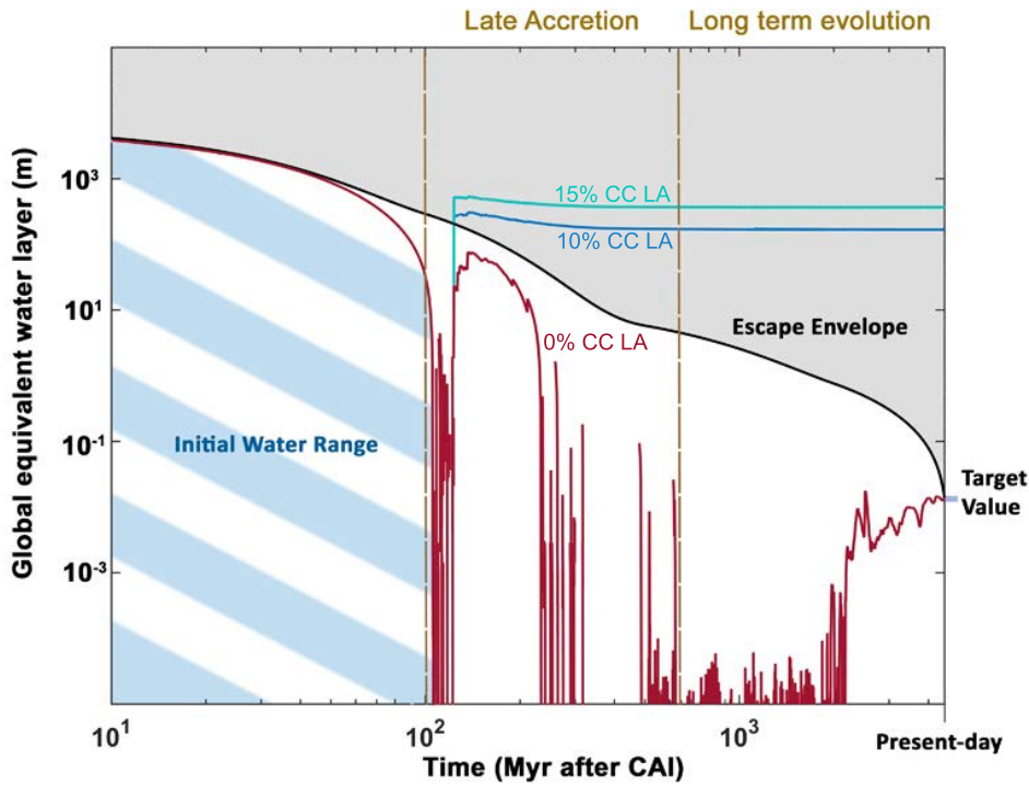
Fig. 11 Evolution of the amount of water at the surface of Venus since its accretion up to present-day, in equivalent global ocean layer depth (adapted from Gillmann et al., 2020). The simulation includes the effects of impacts during late accretion (erosion, delivery, energy transfer), atmospheric escape and volcanism. Three compositions are proposed for the late accretion: fully composed of relatively dry enstatite chondrite-like material (Piani et al., 2020, red line with 0.1% H 2 O, 0.4% CO 2 and 0.02% N 2 ); with 10% wetter material akin to carbonaceous chondrites (blue curve noted CC; by mass, 8% H 2 O, 4% CO 2 and 0.2% N 2 ); and with 15% CC (light blue curve). Only the drier late accretion is consistent with the present-day water inventory in the Venus atmosphere (target value). The escape envelope is the maximum amount of water that could have been present in the atmosphere at a given time and still be consistent with present-day measurements in the absence of all mechanisms other than atmosphere escape. Atmospheric escape is calculated based on Kulikov et al. (2006), and is higher than estimates from Persson et al. (2020). The initial water range illustrates the uncertainty on the water inventory during accretion that is not resolved by the model. Time is measured from the formation of calcium-aluminum rich inclusions (CAIs).
