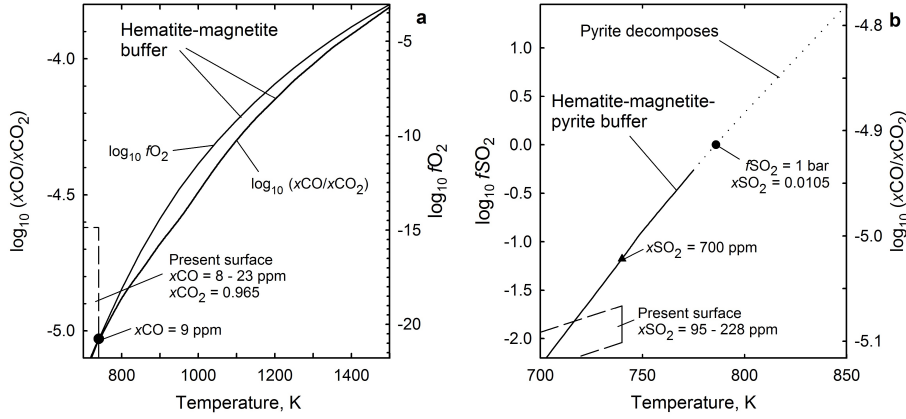
Fig. 7 Possible future changes in concentrations of trace atmospheric gases controlled by mineral-gas equilibria at 95.6 bar. In (a), CO/CO 2 mixing ratio and fO_2 are controlled by the hematite-magnetite equilibrium (Eq. 7) during warming. The area shown by dash lines corresponds to the present near-surface CO/CO 2 ratios (see Fig. 6 for fO_2 ). The circle symbol shows conditions at which CO extrapolated toward the surface (Fegley et al., 1997b; Zolotov, 2019) closely match the equilibrium (Eq. 7). In (b), fugacity of SO 2 is controlled by the hematite-magnetite-pyrite equilibrium at the CO/CO 2 ratio at Eq. (7). The fugacity of SO 2 in the current near-surface atmosphere reflects a range of measured SO 2 concentrations with uncertainties. The triangle symbol shows nominal conditions of the mineral equilibrium at 740 K (see Fig. 6). The circle symbol corresponds to partial pressure of SO 2 of 1 bar at 786 K. The dotted curve shows possible conditions of through decomposition of pyrite in a permeable surface layer. (This figure was developed by M. Zolotov)
