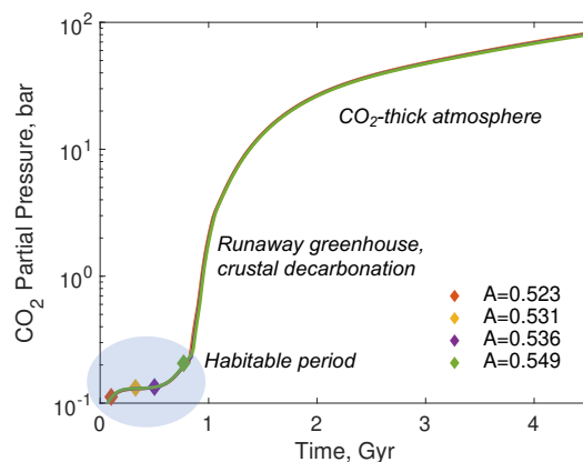
Fig. 9 Modelling results from a coupled interior-atmosphere model of a stagnant lid Venus assuming different planetary albedos, after the solidification of the magma ocean (Höning et al., 2021). The model assumes an initially thin atmosphere containing only the present-day N_2 inventory. Diamonds depict control runs from a 3-D general circulation model (Way et al., 2016; Way and Del Genio, 2020) at the given time (corresponding to incident insolation) and atmospheric CO_2 pressure, yielding the indicated albedo.
