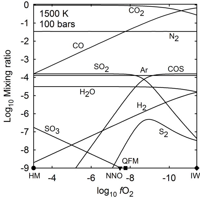
Fig. 8 Mixing ratios of C-O-H-S-N gases with bulk composition of the current atmosphere as functions of fO_2 at 1500 K. The Ar value corresponds to the current atmospheric ^{36}\text{Ar} and ^{38}\text{Ar} contents and tripled current ^{40}\text{Ar} . The figure illustrates possible sequential reduction ( fO_2 decrease) of the atmospheric composition after formation of a second magma ocean on Venus. HM, hematite-magnetite buffer; NNO, Ni-NiO buffer; QFM-quartz-fayalite-magnetite buffer; IW, iron-wüstite buffer. (This figure was developed by M. Zolotov)
