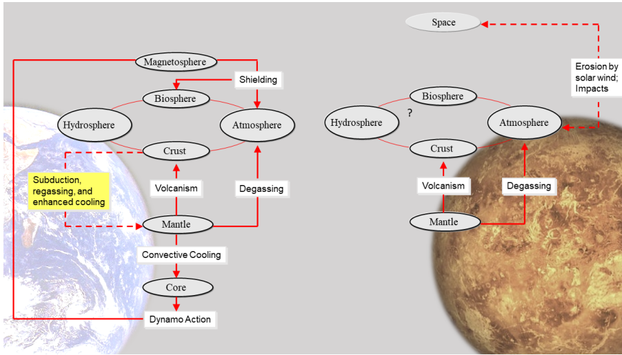
Fig. 1 Sketch of a plate tectonic planet like Earth (left) and a stagnant lid or single plate planet like present Venus (right) showing the interactions between the different reservoirs. Venus shares characteristics with stagnant lid planets but also shows evidence of deformation and horizontal motion. Major difference between plate tectonic planets and stagnant lid planets is the lack of subduction and regassing of volatiles from the surface (i.e., oceanic crust and lithosphere) for the latter. In the plate tectonic scenario, subduction of the cold surface layers (i.e., oceanic crust and lithosphere) leads to efficient cooling of the mantle and core. This can facilitate the generation of a strong magnetic field in the core, which in turn affects atmosphere loss mechanisms caused by the solar wind (see section 3.1 for details). The volatile exchanges in a stagnant lid or a single plate planet are therefore reduced and shows only a one-way path from the mantle into the atmosphere. The reduced volatile circulation may prevent the formation of a biosphere and a hydrosphere over long periods of time. Photos of Earth and Venus in the background, courtesy of NASA/JPL
