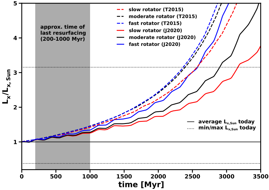
Fig. 3 The evolution of X-ray activity for Sun-like stars normalized to the Sun’s present-day value of 10^{27.2} \text{ erg s}^{-1} \text{ cm}^{-2} according to Tu et al. (2015) (dashed lines) and Johnstone (2020) (solid lines). Red, grey, and blue depict the tracks of initially slow, moderate, and fast rotating Sun-like stars. The evolutionary tracks by Tu et al. (2015) were employed to fit the Sun’s average X-ray flux at present-day, while those by Johnstone (2020) show the respective averages of the rotational tracks for all measured Sun-like stars. The grey shaded area shows the approximate average age of Venus’ surface. As can be seen, this age falls clearly within a time period that can be covered by the variation of the X-ray flux over the solar cycle (solid line for average value, dashed lines for minimum and maximum).
