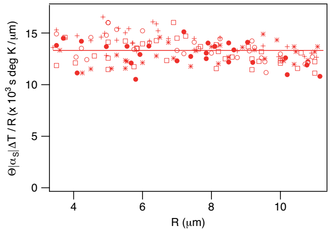
FIG. 25. Combination \Theta\Delta T|\alpha_S|/R as a function of the drop radius R . The symbols for the experimental points are the same as in Fig. 14. This quantity is constant given the dispersion of the data.
