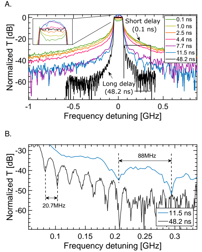
Fig. 5: A. Power transmission T of a 100 MHz wide filter for a wide range of programming delays \tau . The delays are given \pm 0.1 ns;
