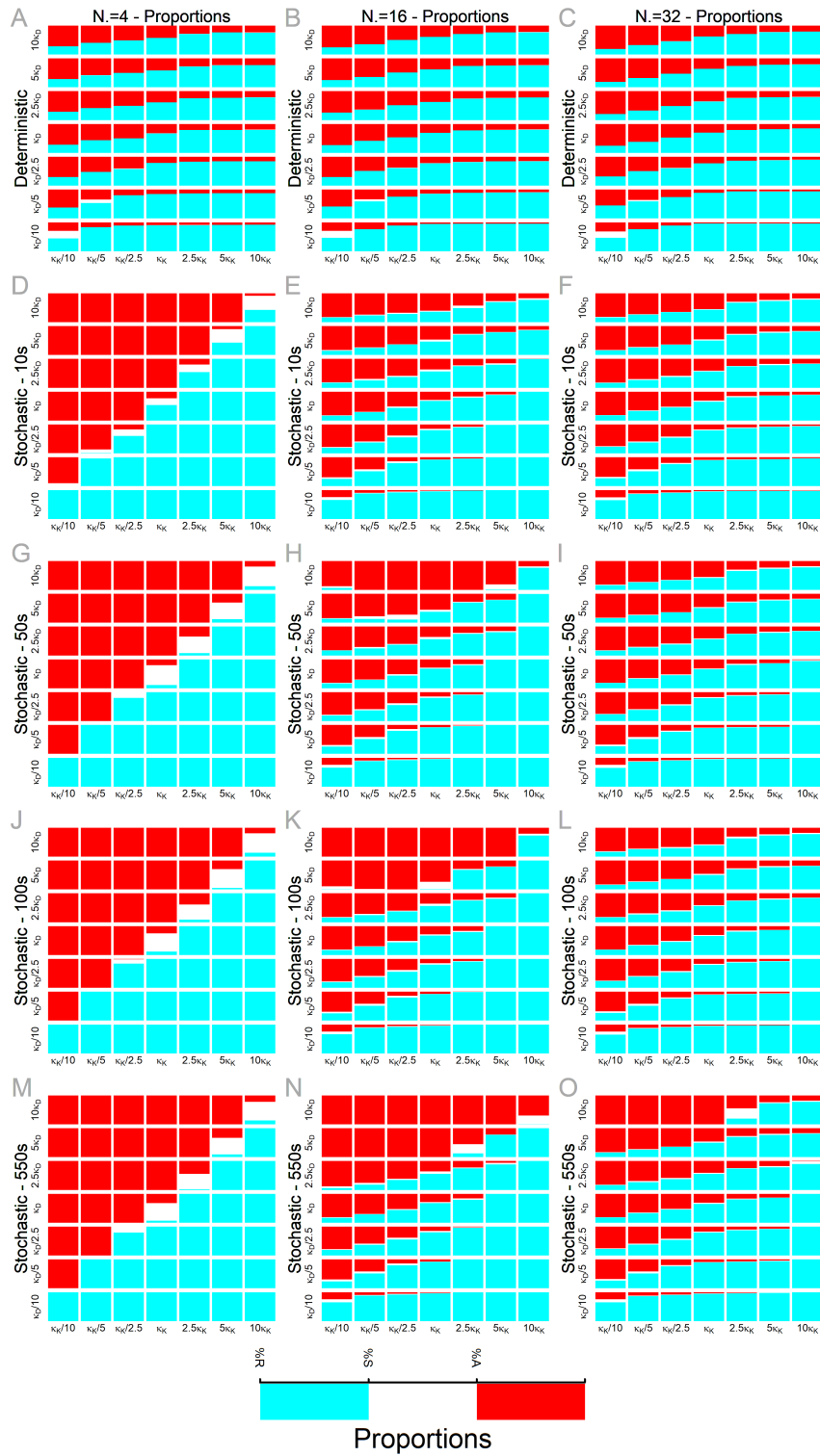
26 Figure 7: Distributions of filaments over different regimes of motion. In each panel, tiles are stacked bar-plots in which proportions of anterograde (in red), slow (in white) and retrograde (in cyan) filaments are represented. Rows and columns are as in Figure 3 and parameter values used for simulations are provided in Table 1.
