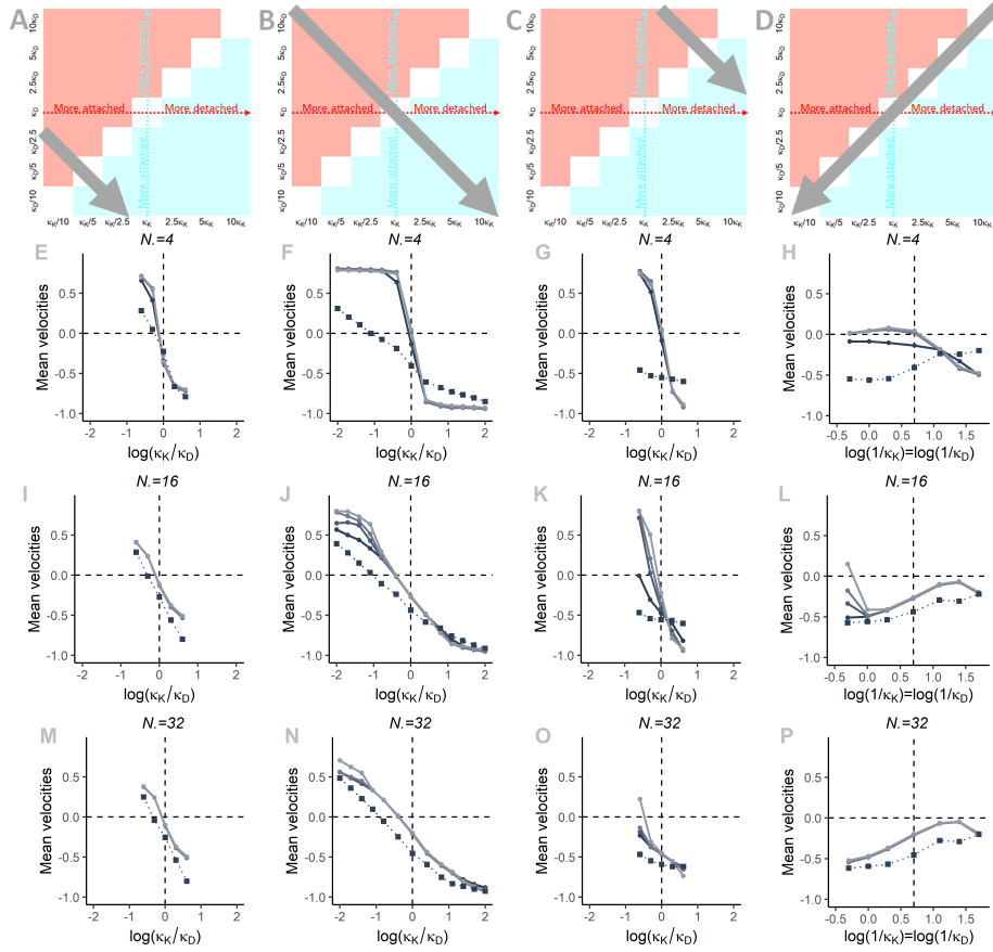
Figure 8: Mean velocities of the 150 filaments as functions of dissociation constant ratios. (A-D) Grey arrows indicated from which regions dissociation constant are taken to compute ratios for each column. Row 2, 3 and 4 show results for N = 4, 16 and 32 . (E, I and M) Both types of motors have dissociation constants smaller than their base values (strong affinities for both motors). (F, J and N) One type with \kappa smaller than its base value and the other with \kappa larger than its base value (one type with a strong affinity and the other with a weak one). (G, K and O) Both types of motors have dissociation constants larger than their base values (weak affinities for both motors). (H, L and P) Both types have the same affinity (from smaller to larger affinities). Dotted lines with squares represent results from the deterministic description and plain lines with dots are results from the stochastic description at different times from 10 seconds (the darkest tone) to 550 seconds (the lightest tone). Parameter values used for simulations are provided in Table 1.
