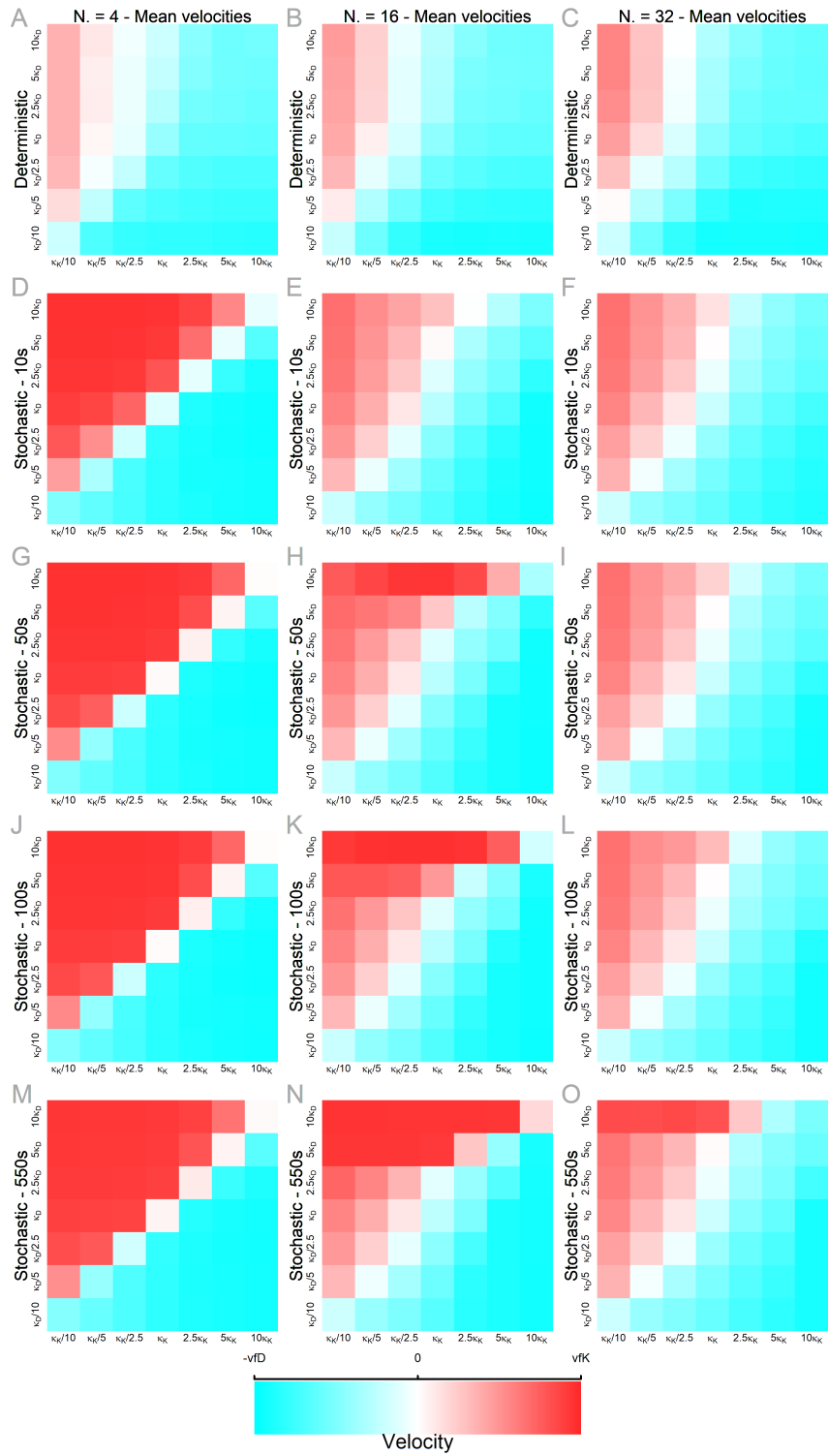
Figure 6: Mean velocities of the 150 filaments. Rows and columns are as in Figure 3 and parameter values used for simulations are provided in Table 1.
