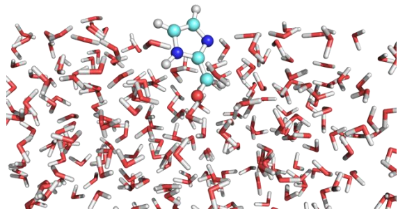
Figure 3. Snapshot from the QM/MM MD simulation of IC( S_0 ) at the air-water interface.
