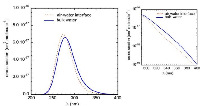
Figure 8. Absorption spectrum of IC in bulk water and at the air-water interface obtained from combined QM/MM MD simulations and MRCI/cc-pVTZ calculations. The inset shows the detail in the tropospheric actinic region in a logarithmic scale.
