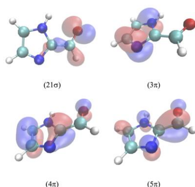
Figure 5. Contour plots of the most significant orbitals of IC calculated in gas phase.
