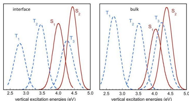
Figure 6. Histograms of vertical excitation energies to the singlet and triplet excited states S_1 , S_2 , T_1 , T_2 and T_3 from S_0 , along the QM/MM MD simulation for IC( S_0 ) at the air-water interface and bulk water. The curves represent Gaussian functions fitting the calculated histograms (see also Figure S3). Average values for S_1 , S_2 , T_1 , T_2 and T_3 are (in eV) 4.06, 4.50, 2.86, 3.52 and 4.31 at the air-water interface, and 4.09, 4.42, 2.81, 3.58 and 4.30 in bulk water, respectively.
