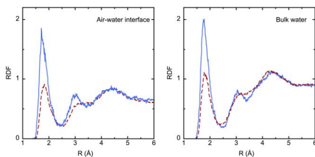
Figure 4. Radial distribution functions (RDFs) for O(IC)...H(water) hydrogen-bond interactions from the QM/MM MD simulations of IC( S_0 ) (dashed red lines) and IC( T_1 ) (plain blue lines) at the air-water interface and in bulk water. The RDFs consider the two H atoms in all water molecules.
