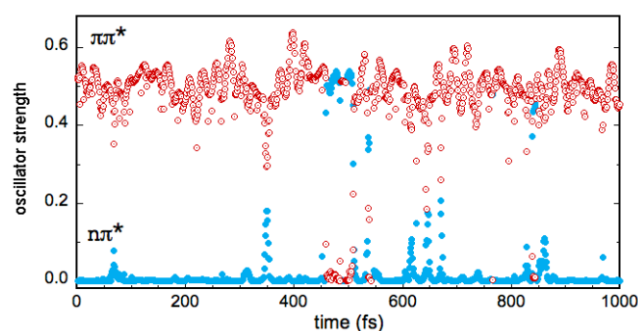
Figure 7. Fluctuations of the oscillator strengths for S_0 \rightarrow S_1 (blue plain circles) and S_0 \rightarrow S_2 (red open circles) electronic transitions along one picosecond of the QM/MM MD simulation of IC in bulk water. The values for transitions with main ( n\pi^* ) or ( \pi\pi^* ) character are indicated.
