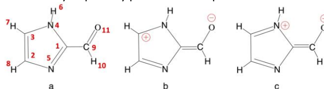
Figure 2. Imidazole-2-carboxaldehyde (IC). Atom numbering used in this work (a), and possible formal mesomeric electronic structures for the \pi system (b and c).
