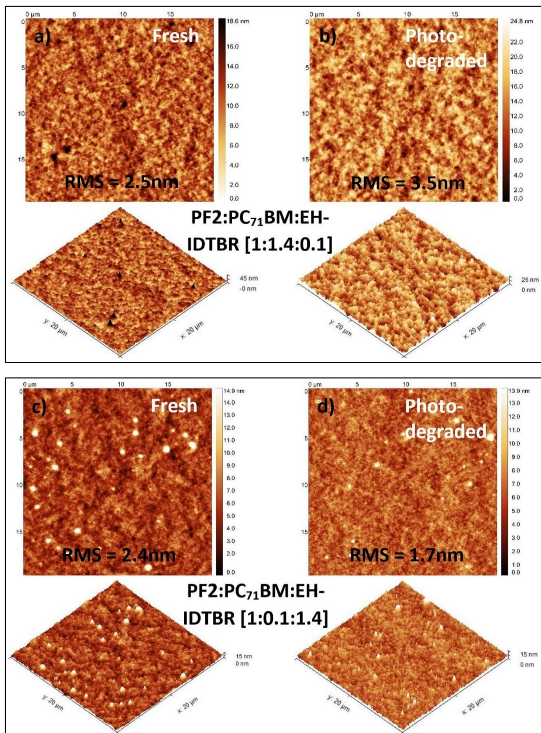
Fig. 10. (1.5 column) Atomic force microscopy (AFM) topography images (20 μm × 20 μm) before degradation a) and c) and after LED continuous illumination for three hours b) and d) for [PF2:PC 71 BM:EH-IDTBR] devices with [1:1.4:0.1] and [1:0.1:1.4] mass ratio, respectively. RMS stands for Root Mean Square rugosity.
