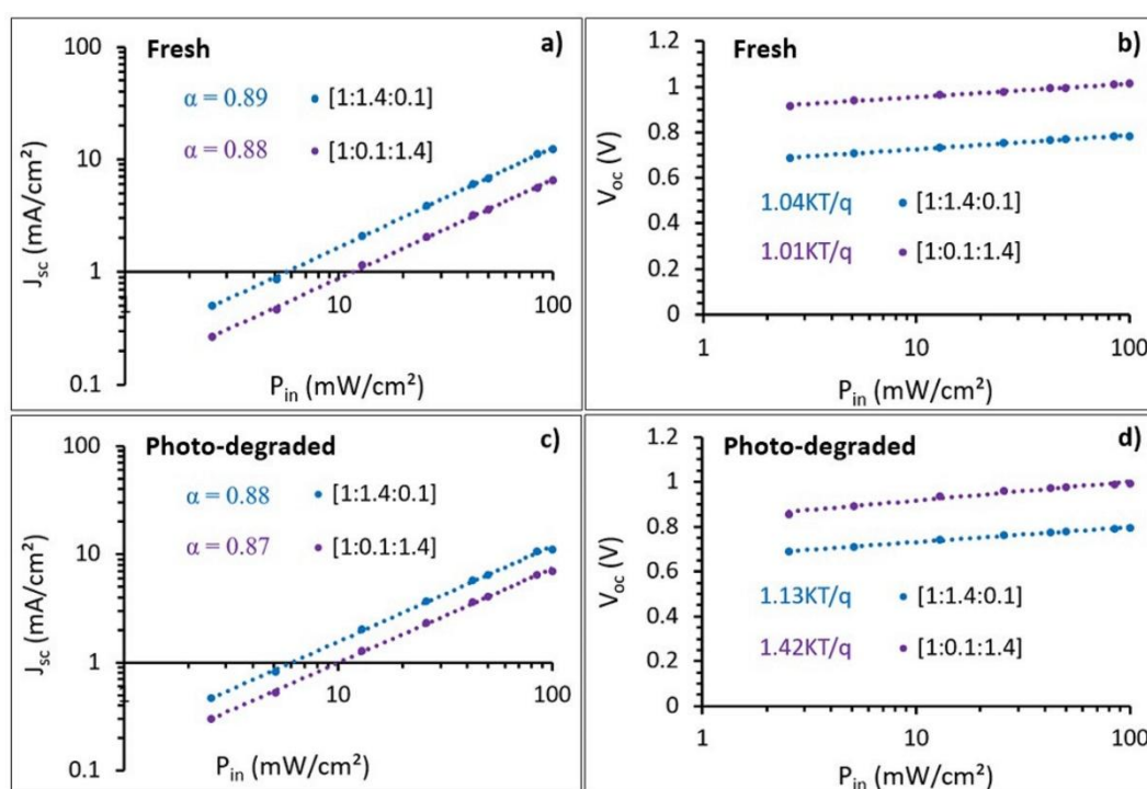
Fig. 9. (1.5 column) Light intensity ( P_{in} ) dependence of short-circuit current ( J_{sc} ) and open-circuit voltage ( V_{oc} ), respectively, a) and b) before photo-degradation, c) and d) after photo-degradation. Measurements were performed on 12 mm 2 photodiode area in the inverted structure.
