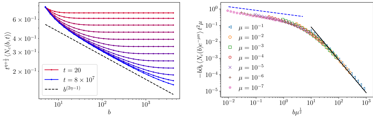
FIG. 5. Results obtained from numerical integration of the KPP equation. Left panel: Average cluster number, with the predicted t dependence removed, t^{\eta+1/2} \langle N_c(b) \rangle , for b \in [5, 5000] and t = 20, \dots, 8 \times 10^7 (represented by color, from red to blue). The dashed line indicates the b^{2\eta-1} ( \eta = 0.39 ) prediction, with arbitrarily adjusted prefactor. Right panel: Testing the prediction (61) on the cluster number with particle number conditioning, for a few values of \mu . The value of t alternates between 3.3 \times 10^8 and 1.3 \times 10^9 . The blue dashed line plots the power laws (b \mu^{1/2})^{2\eta-1} with an arbitrarily adjusted prefactor. The black solid lines depicts 8(b \mu^{1/2})^{-2} with the predicted exact prefactor. See Appendix E2 for numerical methods.
