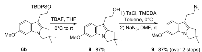
Scheme 5 Functional group interchange of pyrrolo[1,2- a ]indole 6 .
