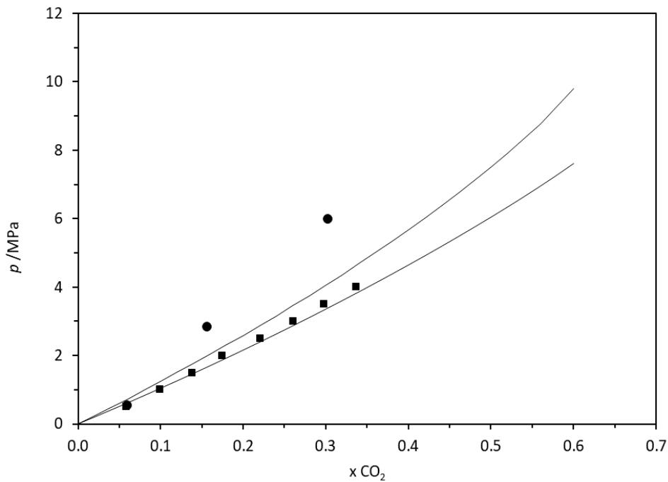
Figure 7. Solubility of CO 2 in cyrene: ■ 313 K (this work); ● molecular simulation at 323.5 K ; — SRK ( k_{ij} = -0.13009 ).
