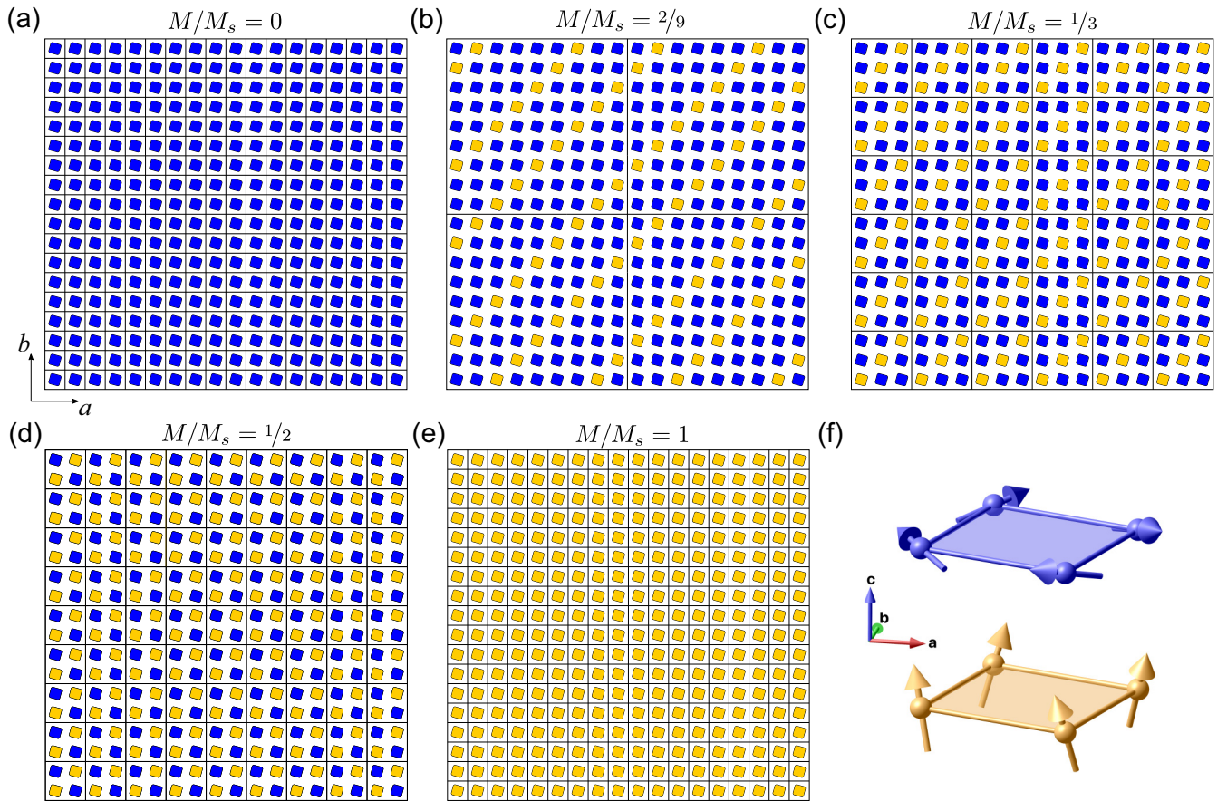
FIG. 6. Magnetic structure models for the different phases in \text{TbB}_4 , where a blue (orange) square represents a 4-spin plaquette with magnetic moments within (perpendicular to) the a - b plane. Black lines denote the magnetic unit cells. (a) Zero-field magnetic structure with all magnetic moments lying within the a - b plane. (b) 2/9 -magnetization plateau phase with a 9 \times 9 supercell, in which polarized spin-plaquette stripes are alternately separated by three or four nonpolarized stripes (note that this separation cannot be deduced from the data at hand and that this illustration would correspond to repelling polarized stripes). (c) 1/3 -magnetization phase with a 3 \times 3 supercell featuring polarized plaquettes along the diagonal of each magnetic unit cell. (d) 1/2 -magnetization phase with a 2 \times 2 supercell. (e) Fully polarized state with magnetic moments along the c axis. Note that in (b)–(d) the magnetic moments represented by blue (orange) squares do not lie fully within (perpendicular to) the a - b plane and that they produce superstructure reflections at \mathbf{Q} = (1/9 \ 1/9 \ 0) , \mathbf{Q} = (1/3 \ 1/3 \ 0) , and \mathbf{Q} = (1/2 \ 1/2 \ 0) , respectively, expressed with the conventional 1 \times 1 unit cell. (f) Detailed view on two 4-spin plaquettes used as building blocks in the models (a)–(e). The upper (blue) one consists of magnetic moments predominantly aligned in the a - b plane with a nonzero ferromagnetic c component for the intermediate structures, while the lower (orange) one is almost fully polarized in (b)–(d) and fully polarized in (e).
