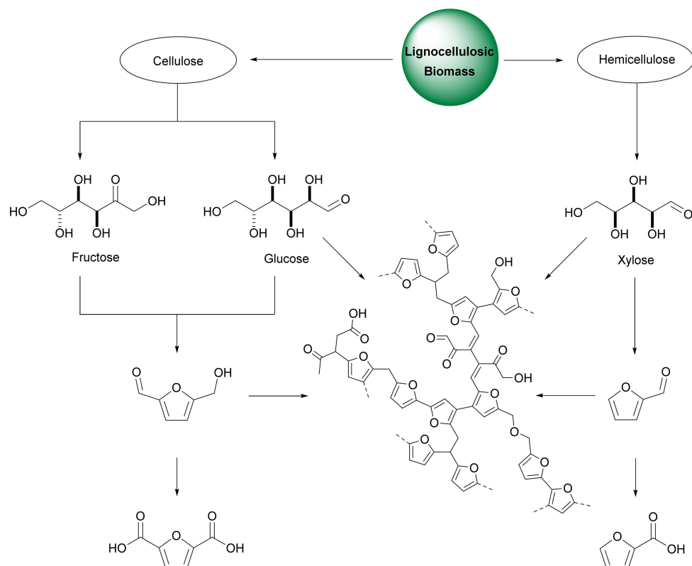
Scheme 11. Synthesis of humin by-product from conversion of lignocellulosic biomass to platform chemicals.
