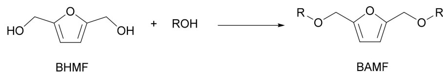
Scheme 10. Etherification via dehydration of 2,5-bis(hydroxymethyl)furan (BHMF) with alcohol to 2,5-bis(alkoxymethyl)furan (BAMF).
