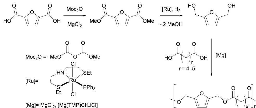
Scheme 9. One-pot catalytic approach to BHMF-based polyesters from FDCA.
