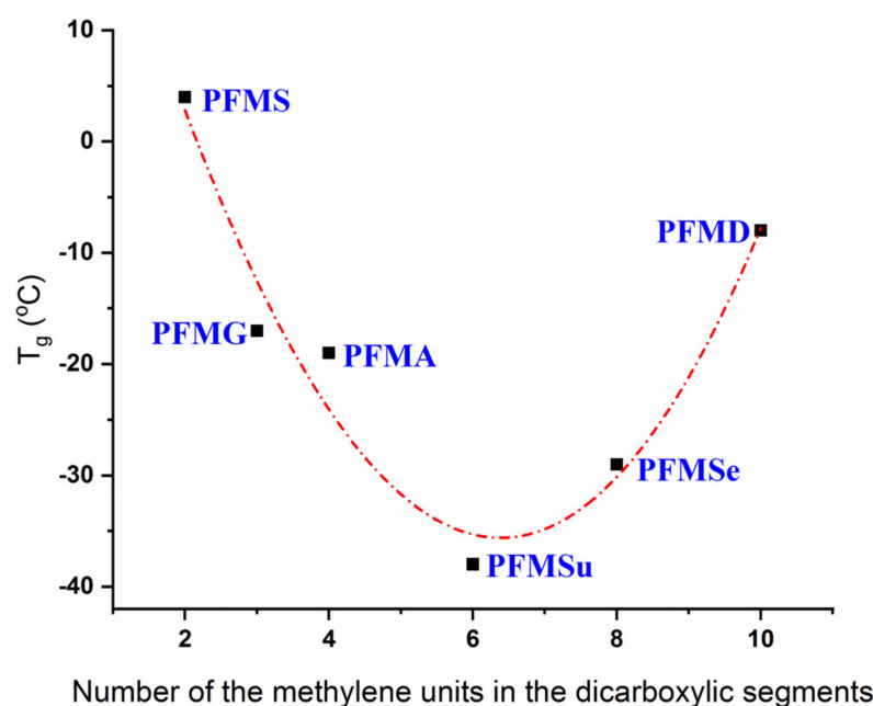
Figure 6. Glass transition temperature of 2,5-bis(hydroxymethyl)furan-based polyesters of increasing diacid chain length. Reprinted with permission from reference [41]. Copyright 2014 American Chemical Society.
