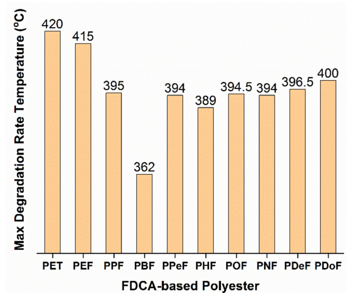
Figure 4. Temperature at which maximum degradation rate is achieved for each polyester (based on data from references [26–28]).
