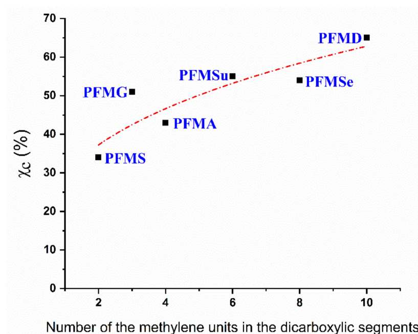
Figure 5. Degree of crystallinity ( \chi_c ) of the 1,5-bis(hydroxymethyl)furan-based polymers with varying number of methylene units in the diacid ethyl esters. Reprinted with permission from reference [41]. Copyright 2014 American Chemical Society.
