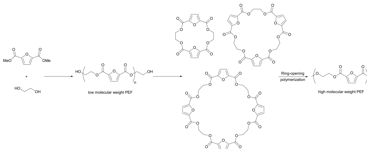
Scheme 7. Polymerization of ethylene glycol and the dimethyl ester of 2,5-furandicarboxylic acid to poly(ethylene) furanoate (PEF) oligomers and final ring-opening polymerization to PEF.
