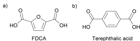
Figure 1. Chemical structures of (a) 2,5-furandicarboxylic acid and (b) terephthalic acid.
