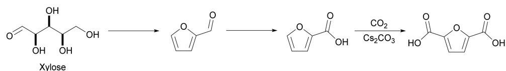
Scheme 4. Carboxylation of 2-furancarboxylic acid to 2,5-furandicarboxylic acid.
