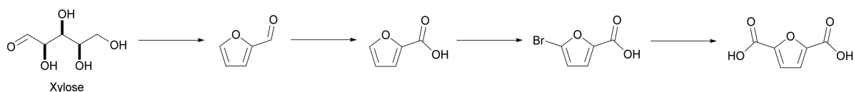
Scheme 3. Bromination of 2-furancarboxylic acid to 5-bromofuroic acid and subsequent reductive carbonylation to 2,5-furandicarboxylic acid.
