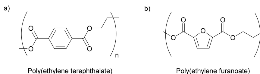
Figure 3. Chemical structure of (a) poly(ethylene terephthalate) (PET) and (b) poly(ethylene furanoate) (PEF).
