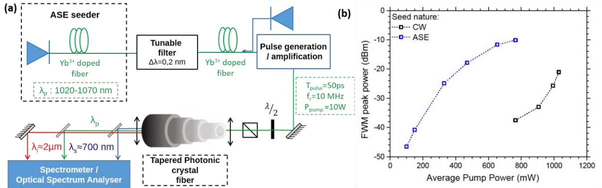
Fig. 1 (a) Experimental scheme of the PCF characterisation source. (b) Evolution of the signal power generated through FWM as a function of the pump power for an ASE seed or a Continuous Wave seed.
