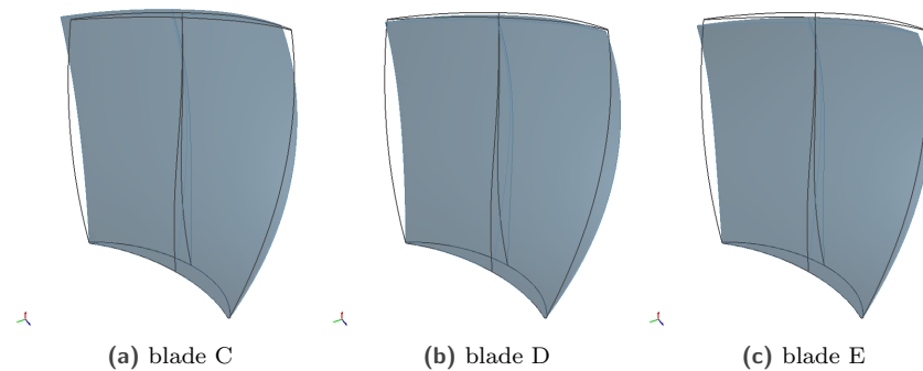
Figure 14. CAD models of optimized blades ( \blacksquare ) with respect to initial rotor 67 blade ( \square ).
