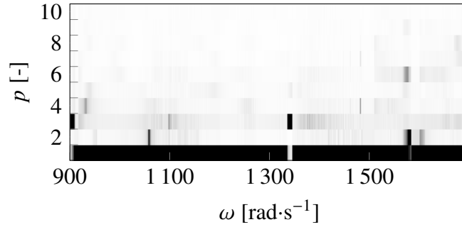
Figure 13. Normalized modal contributions of initial blade rotor 67 (from 0 ( \square ) to 1 ( \blacksquare )).
