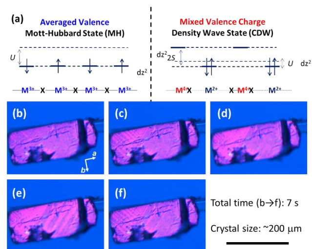
Figure 1. (a) Electronic state of quasi-one-dimensional halogen-bridged metal complexes. (b-f) Phase separation between MV-CDW and AV-MH at 141 K in fluctuating N 2 gas flow (See movie 1)
