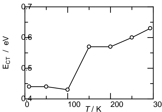
Figure 8. E_{CT} vs. T plots of 1 at various temperatures.
