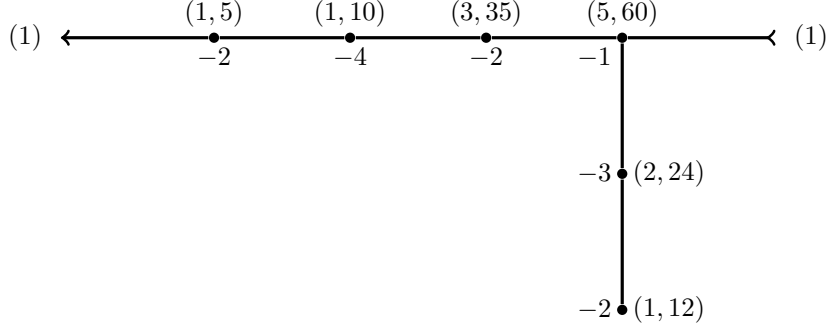
FIGURE 6. The numbers between parenthesis are the orders of vanishing (m_v(g), m_v(f)) of the functions g \circ \pi and f \circ \pi along the irreducible components of E , these numbers can be determined from the dual graph using Proposition 1.3.
