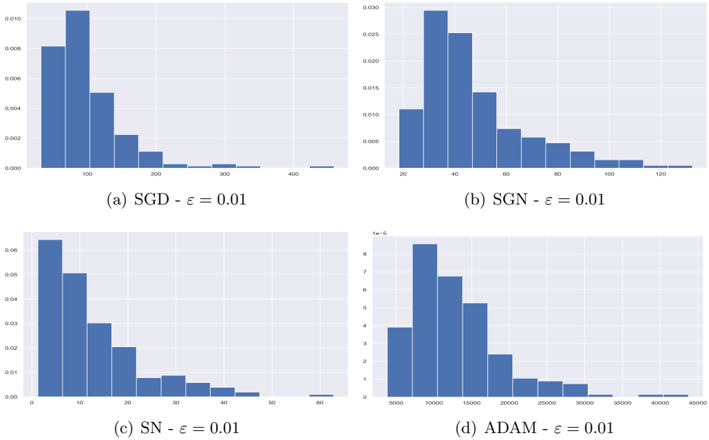
Figure 9: Discrete setting with I = 10^3 , J = 50 and \varepsilon = 0.01 . Histogram of 200 independent realizations of n\|\widehat{V}_n - v^*\|^2 with n = 4 \times 10^5 iterations using each of the four stochastic algorithms.
