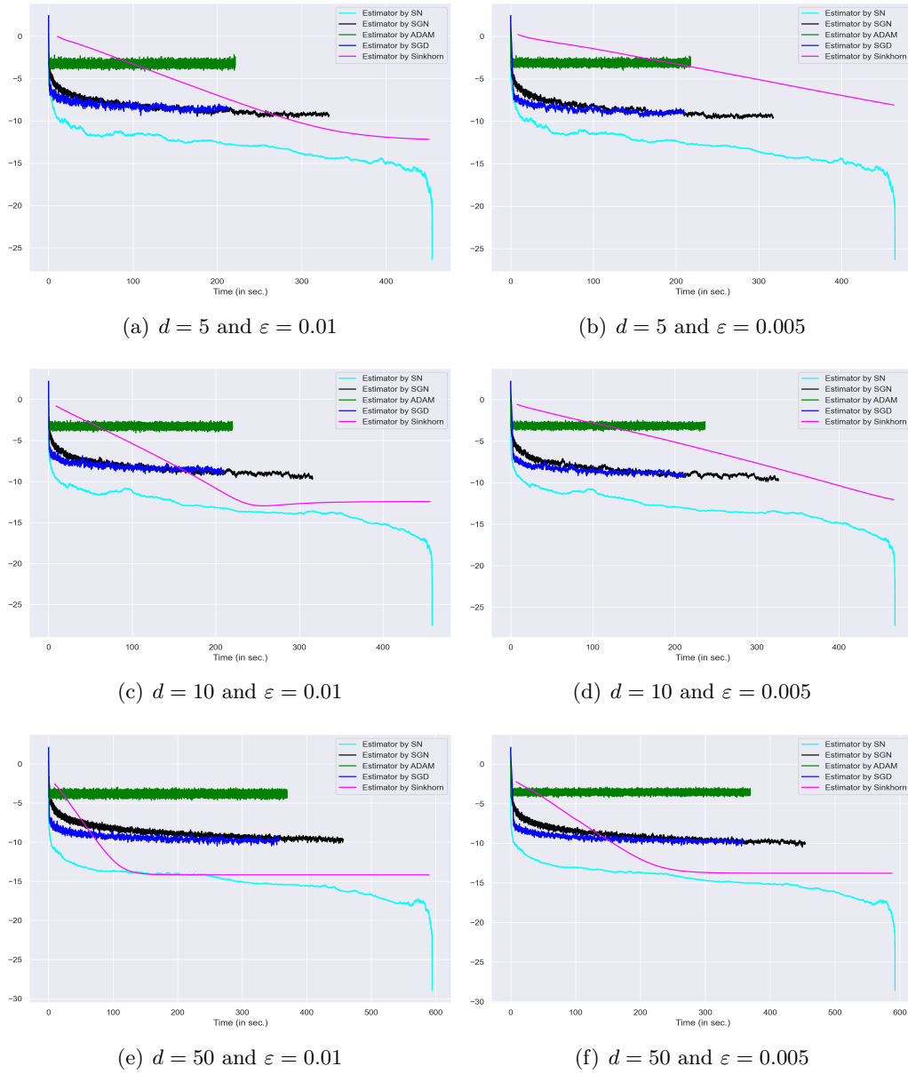
Figure 12: Semi-discrete setting where \mu is a mixture of three Gaussian densities, J = 100 and n = n_{\max} = 10^6 iterations. Excess risk (in logarithmic scale) \log(\|\hat{V}_n - v^*\|^2) (resp. metric \log(\|V_k - v^*\|^2) ) as a function of the computational cost of the iterations of the four stochastic algorithms (resp. the Sinkhorn algorithm) for different values of the dimension d and the regularization parameter \epsilon .
