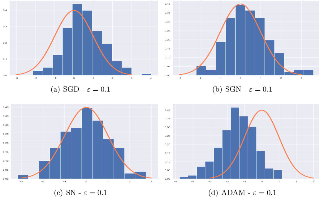
Figure 6: Discrete setting with I = 10^3 , J = 50 and \varepsilon = 0.1 . Histogram of 200 independent realizations of \frac{\sqrt{n}(\widehat{W}_n - W_\varepsilon(\mu, \nu))}{\widehat{\sigma}_n} with n = 2 \times 10^5 using each of the four stochastic algorithms. The orange curve is the density of the standard Gaussian distribution.
