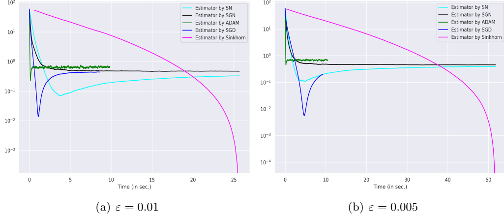
Figure 5: Discrete setting with I = 10^4 and J = 400 with n = 10^5 iterations. Expected excess risk (in logarithmic scale) \log(\mathbb{E}[\|\widehat{V}_n - v^*\|^2]) (resp. metric \log(\|V_k - v^*\|^2) ) as a function of the averaged computational cost of the iterations of the four stochastic algorithms (resp. the Sinkhorn algorithm) for different values of the regularization parameter \varepsilon .
