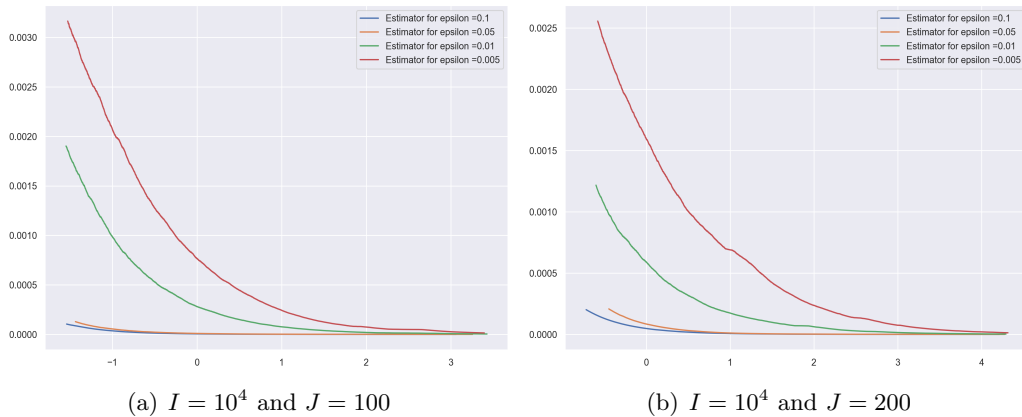
Figure 10: Discrete setting and convergence of \log \left( \|\bar{S}_n - G_\varepsilon(v^*)\|_F^2 \right) as a function of the computational time of the SGN algorithm (using n = 10^5 iterations) for different values of the regularization parameter \varepsilon .
