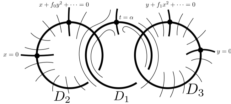
FIGURE 3.1. Topology of the leaves of the vector field (X_1 + X_2)^E
