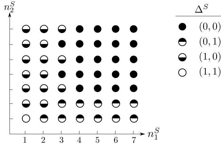
FIGURE 5.1. Unique admissible choice of \Delta^S = (\Delta_1^S, \Delta_2^S) .
