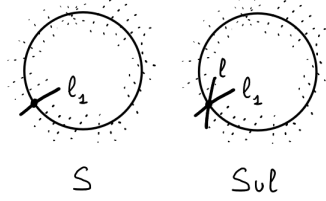
FIGURE 3.2. Topology of the Saito vector fields of S and S \cup l .
