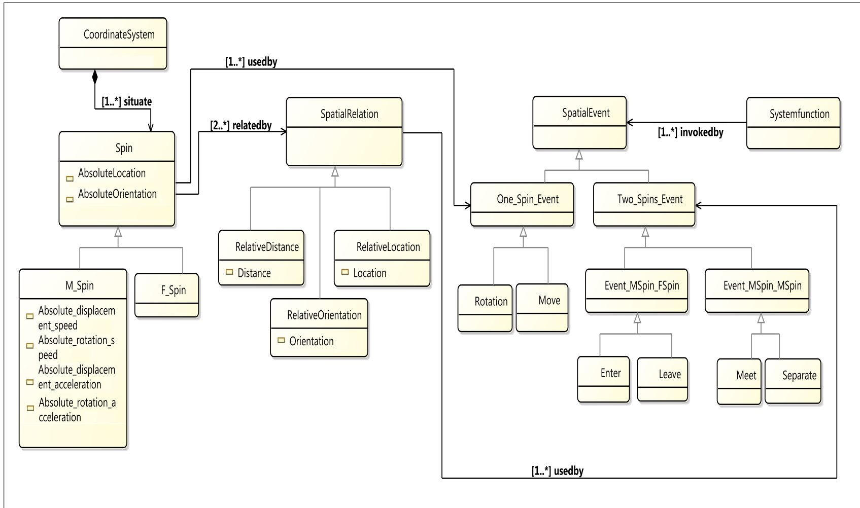
Figure 2: Global view of the SUIL metamodel.
