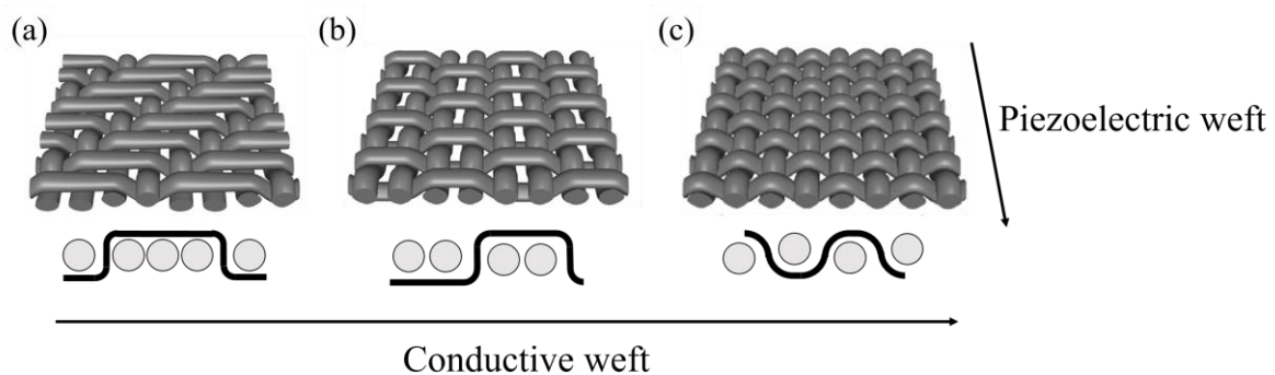
Figure 18. Three different woven patterns made from PVDF and carbon black/polyethylene coaxial fibers (piezoelectric weft) and different conductive yarns. a) Twill b) Weft rib c) plain weave. Adapted from 200 with permission.
