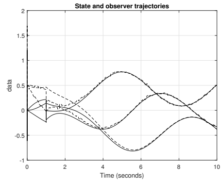
Fig. 1: system states (plain), estimated states (dashed)
