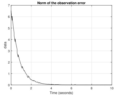
Fig. 2: Norm of the estimation error \|x(t) - \hat{x}(t)\|
