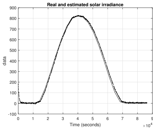
Fig. 3: solar irradiance (plain), estimated solar irradiance (dashed)
