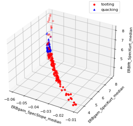
(a) Top-3 most relevant timbre features
