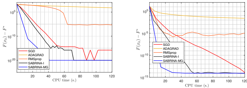
Fig. 1: Evolution of the objective function along time for various algorithms, on dataset rcv1 (left) and a8a (right). Noise amplitude C = 0.95 \times C_{\max} .
