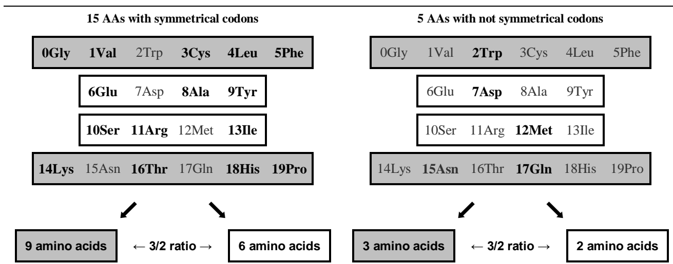
Fig. 47 Distribution in 3/2 ratios of the two AA sets at symmetrical codons (same 1 st and 3 rd identical nucleobases) or at not symmetrical codons according to predefined numbering zones.
