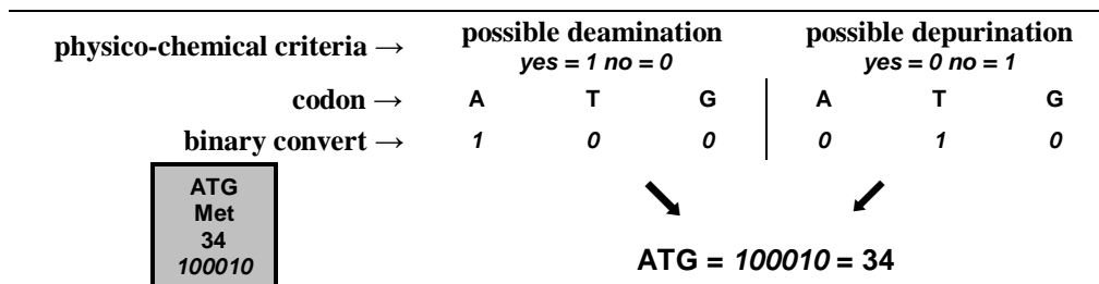
Fig. 2 Method of assigning a number to codons according to Sergey Petoukhov. See Fig. 1 and 3 also.
