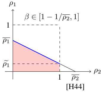
Fig. 6. The five cases that can arise under [H4]: the feasible set is depicted in red. The Pareto boundary in cases [H42]-[H44] is the blue segment given by \rho_1 = \beta \bar{\rho}_1 ; \rho_2 = (1 - \beta) \bar{\rho}_2 .
