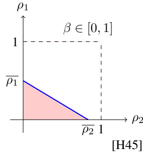
Fig. 6. The five cases that can arise under [H4]: the feasible set is depicted in red. The Pareto boundary in cases [H42]-[H44] is the blue segment given by \rho_1 = \beta \bar{\rho}_1 ; \rho_2 = (1 - \beta) \bar{\rho}_2 .
