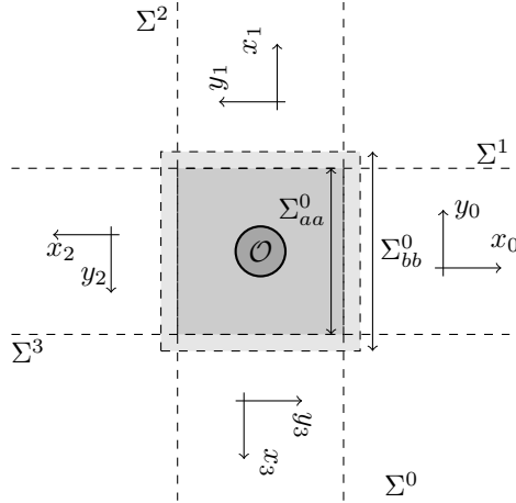
Figure 3: Notations : the domain \Omega_b is the largest square represented in light gray and the domain \Omega_a is the interior square in stronger grey. The obstacle \mathcal{O} is represented by the small circle in the strongest gray.
