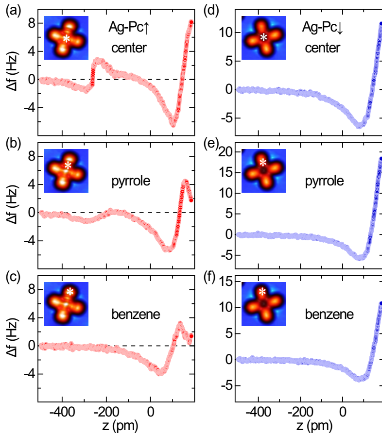
Figure 4: Spatially resolved short-range resonance frequency changes as a function of the tip excursion. (a)–(c) \Delta f(z) acquired atop Ag-Pc \uparrow at the Ag center, the center of the pyrrole and benzene moieties. Inset: STM image of Ag-Pc \uparrow (50 mV, 15 pA, 2 nm \times 2 nm) with indicated (asterisk) position of the \Delta f(z) measurement. (d)–(f) Same as (a)–(c) for Ag-Pc \downarrow .
