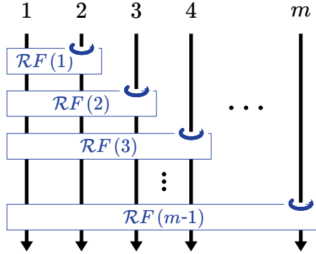
FIGURE 19. The Habegger–Lin decomposition in terms of clasper.
