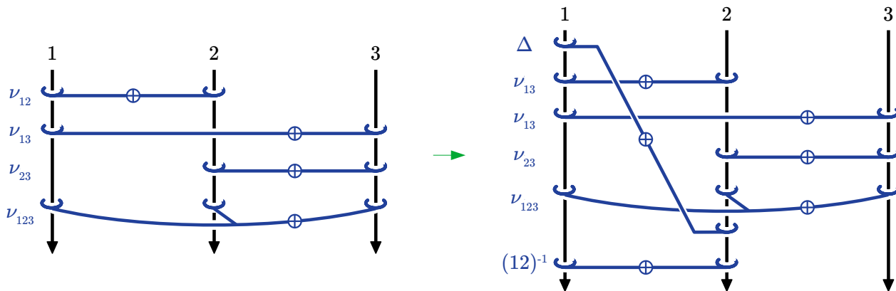
FIGURE 23. The 1-th partial conjugation by x_2 on the normal form.
