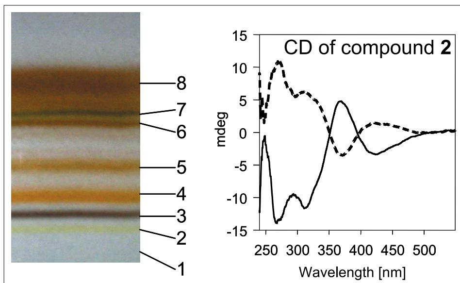
Fig. 6. Left: Polyacrylamide gel electrophoresis (PAGE) separation of N-isobutyryl-L-cysteine protected gold particles. The separation was performed for 17 h at 150 V. The separated compounds are numbered from 1–8 according to their decreasing electrophoretic mobility. Compound 1 is only visible under UV irradiation. Right: CD spectra of separated compound 2 of gold particles covered with N-isobutyryl-L-cysteine (dashed) and N-isobutyryl-L-cysteine (solid line). Adapted with permission from [21]. Copyright (2005) American Chemical Society.
