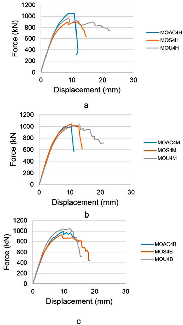
Figure 4. Force-displacement curves for the (a) upper (b) middle and (c) lower portions
