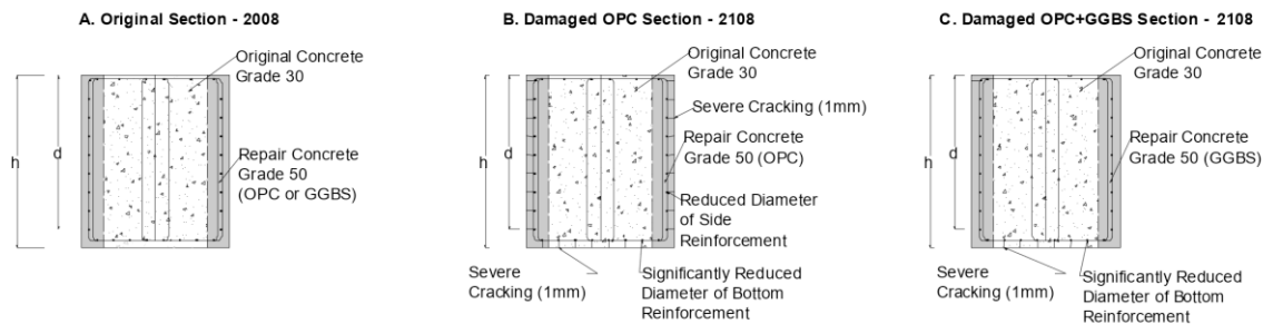
Fig. 1. Cross-sections modelled in structural analysis
