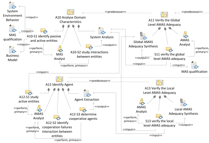
Fig. 27 The Analysis Phase Described in terms of Activities and Work P products
