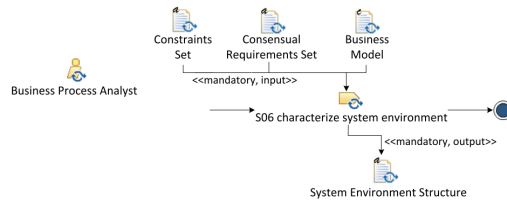
Fig. 19 Flow of Tasks of the Characterize System Environment Activity
