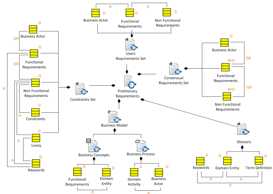
Fig. 15 The Preliminary Requirements Documents Structure
