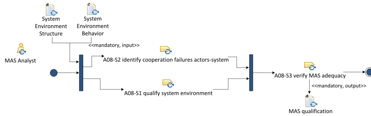
Fig. 21 Flow of Tasks of the Verify MAS Adequacy Activity
