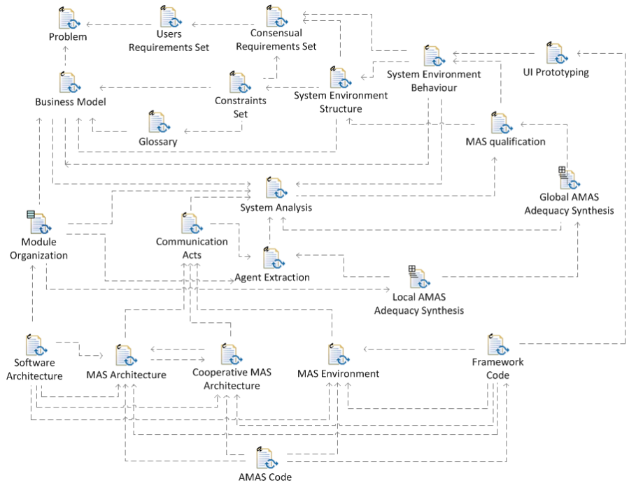
Fig. 53 The Work Products Dependencies
