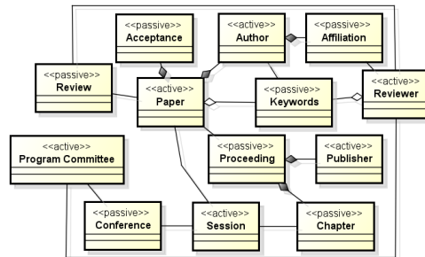
Fig. 33 Entities Structure System Diagram
