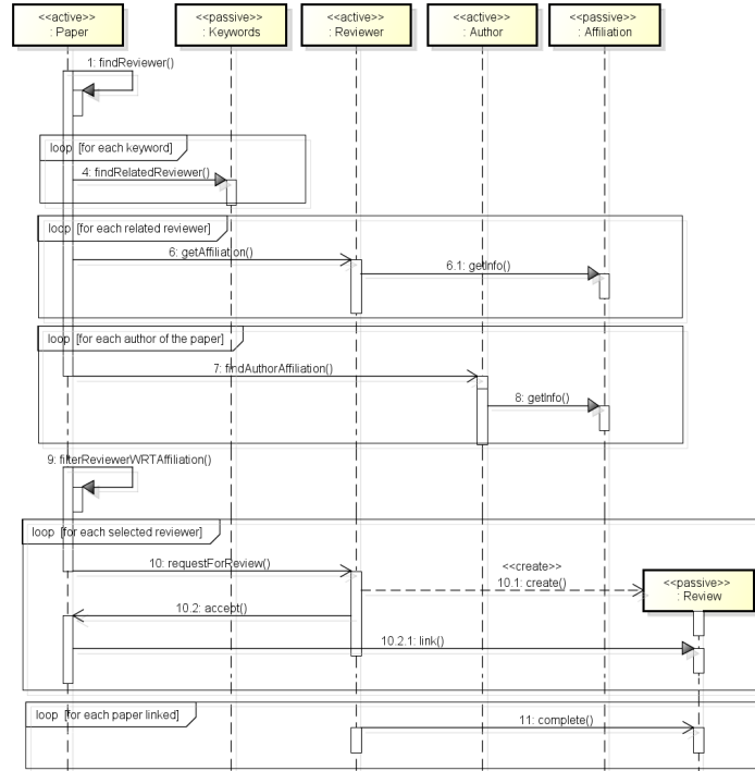
Fig. 34 Entities Interactions System Structure (beginning)
