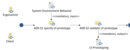
Fig. 22 Flow of Tasks of the Elaborate UI Prototypes Activity
