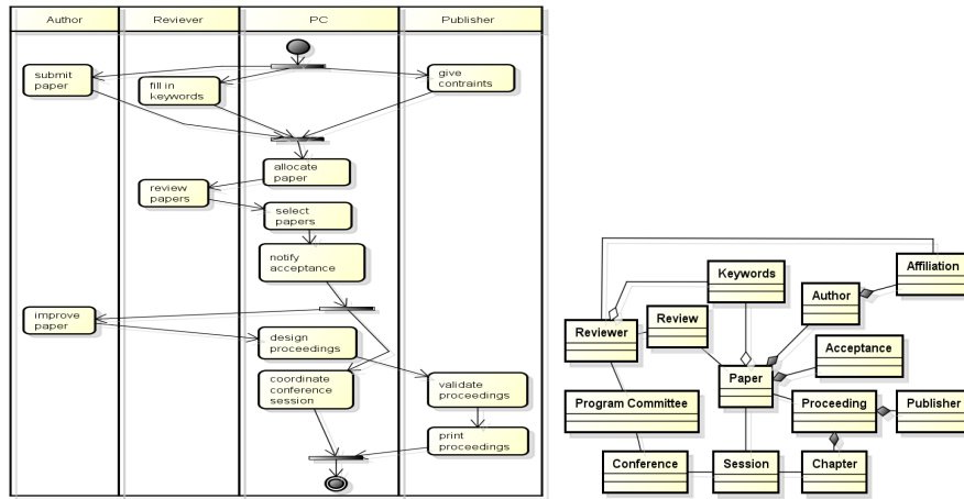
Fig. 16 Business Process (left); Business Concepts (right)
