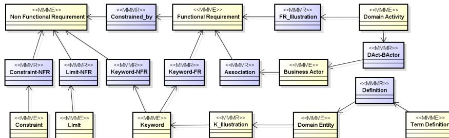
Fig. 2 The Preliminary Requirements Phase MAS Metamodel
