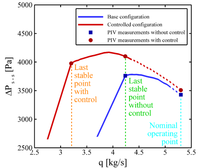
FIGURE 4: PERFORMANCE CURVES OF THE COMPRESSOR WITH PIV MEASUREMENTS IN BASE AND CONTROLLED CONFIGURATIONS
